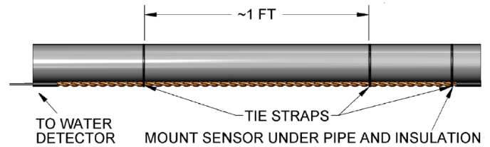
Figure 8: Horizontal Pipe Rope Sensor Mounting
