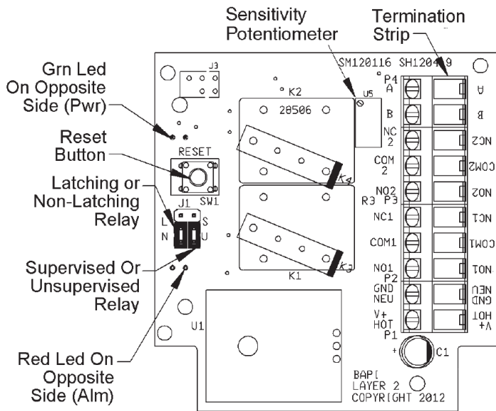
Figure 10: Leak Detector Circuit Board
