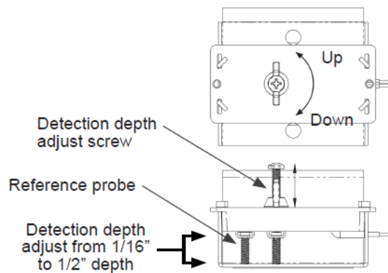
Figure 5: Remote Spot Sensor Depth Adjust
