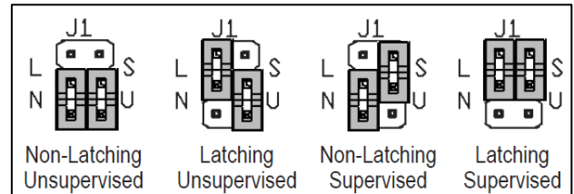
Figure 13: Jumper J1 Settings
