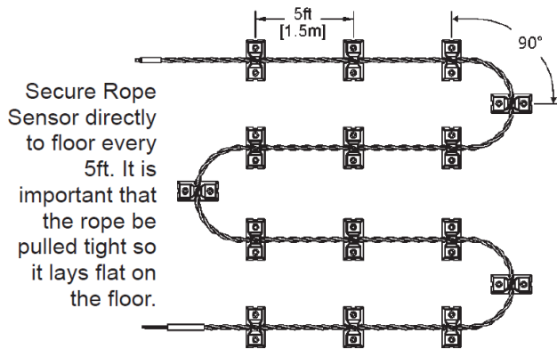
Figure 7: Sub-Floor Rope Sensor Mounting
