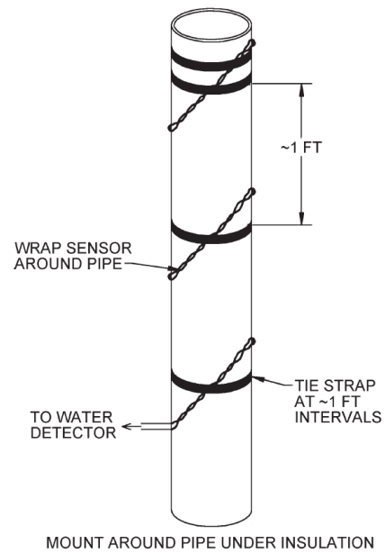
Figure 9: Vertical Pipe Rope Sensor Mounting
