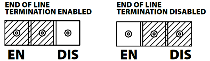
Figure 5: EOL Termination Jumpers
