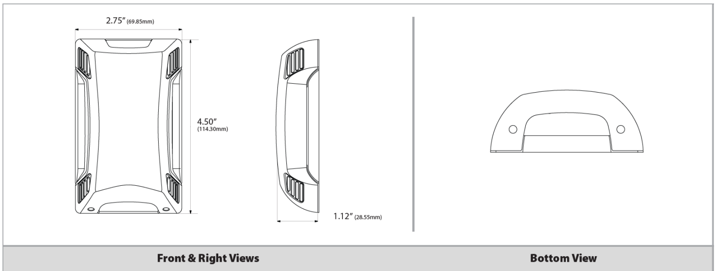
Figure 1: Dimensional Drawing
