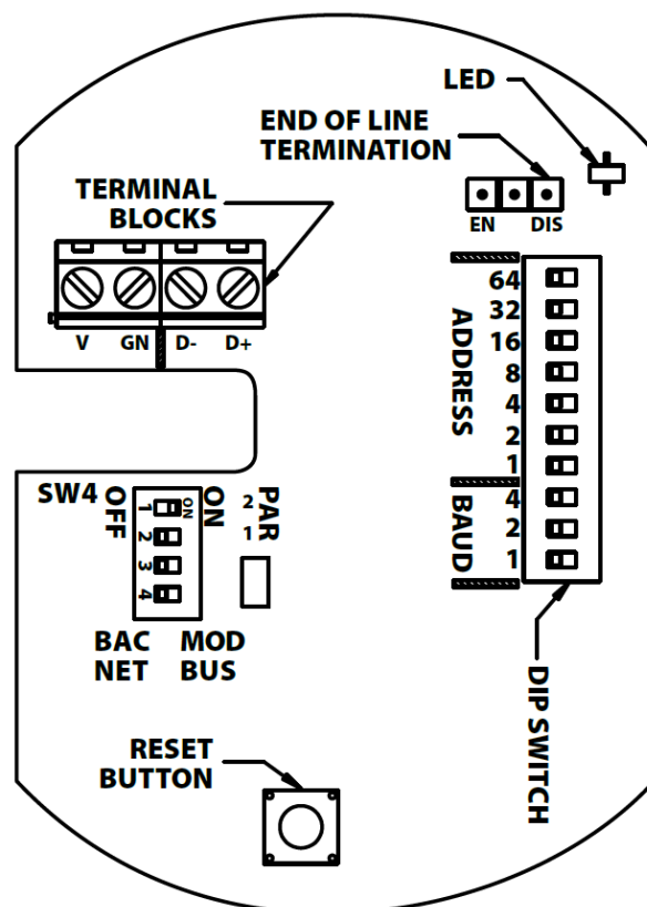
Figure 3: Wiring Diagram
