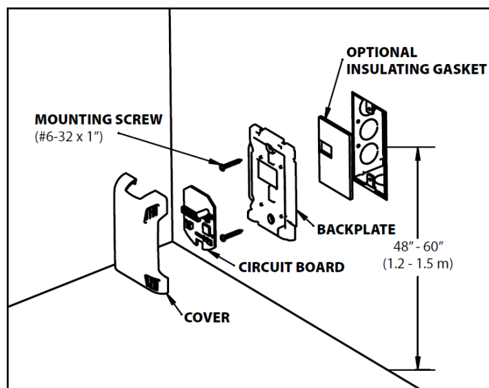
Figure 2: Mounting Diagram
