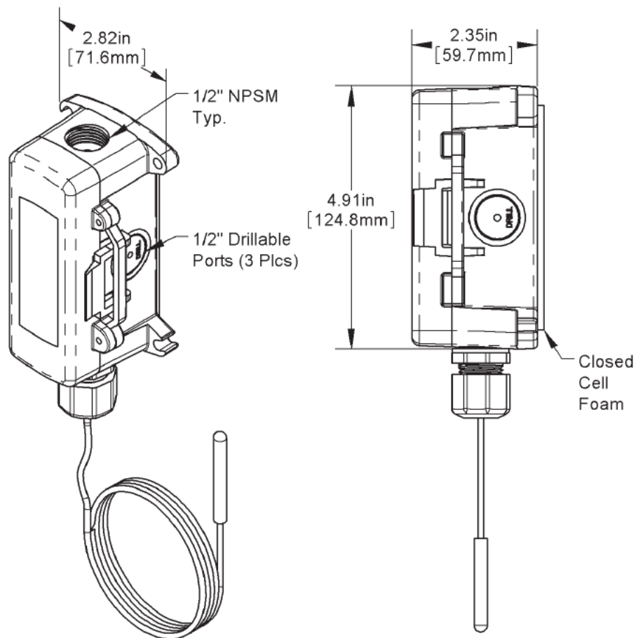
Figure 1: BBox2 (BB2) Enclosure
