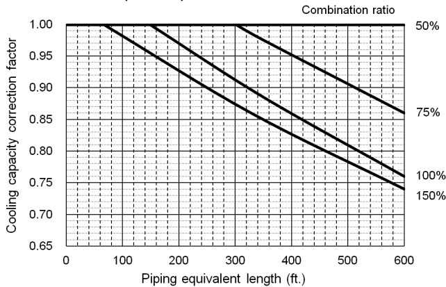
38VMA240RDL5-1(RDS6-1)
