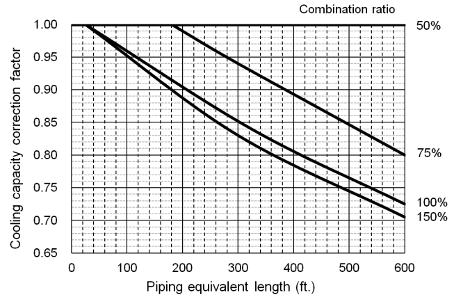
38VMA240RDS5-1(RDS6-1)
