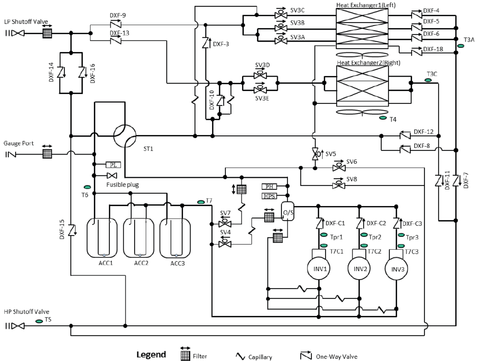
Fig. 9 —38VMA240RDL, 264, 288, 312, 336RDS Models
