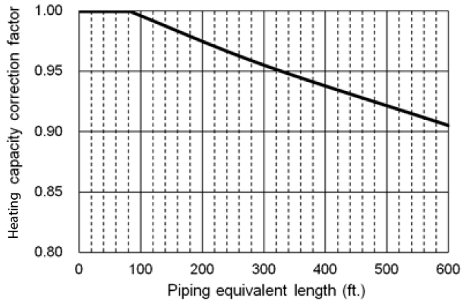
38VMA312RDS5-1(RDS6-1)
