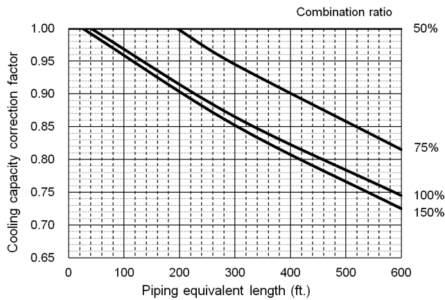
38VMA216RDS5-1(RDS6-1)
