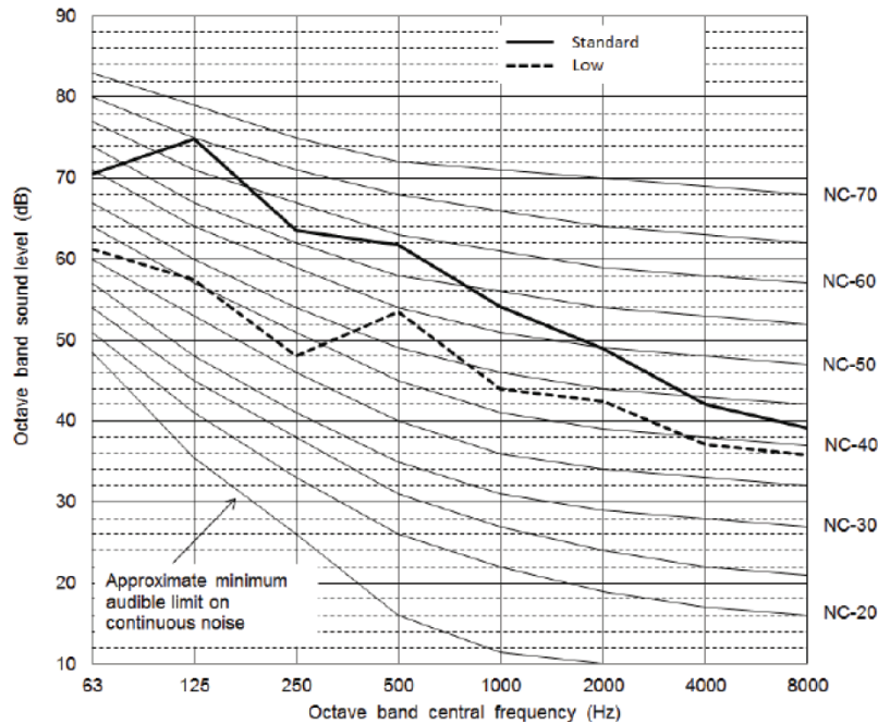
Fig. 30 —38VMA144RDL6-1
