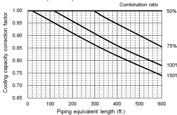
38VMA336RDS5-1(RDS6-1)
