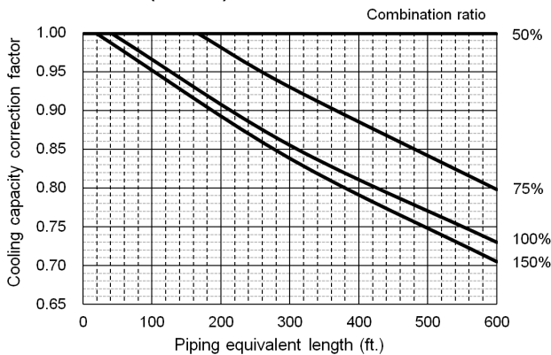
38VMA336RDS5-1(RDS6-1)
