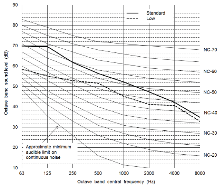
Fig. 25 —38VMA096RDS5-1
