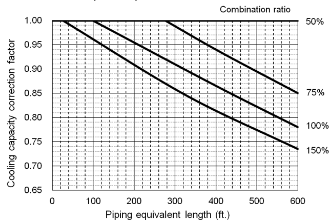
38VMA096RDS5-1(RDS6-1)
