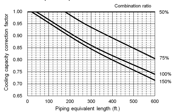
38VMA312RDS5-1(RDS6-1)
