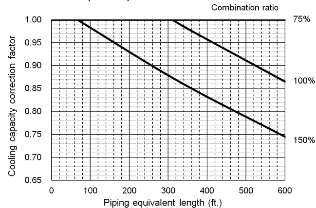
38VMA144RDL5-1(RDL6-1)
