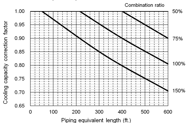
38VMA072RDS5-1(RDS6-1)
