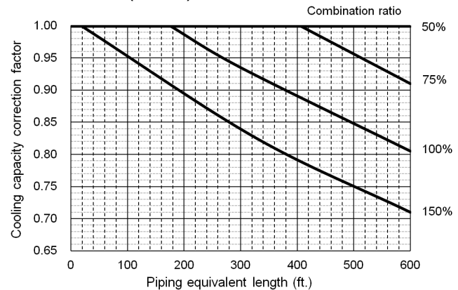
38VMA264RDS5-1(RDS6-1)
