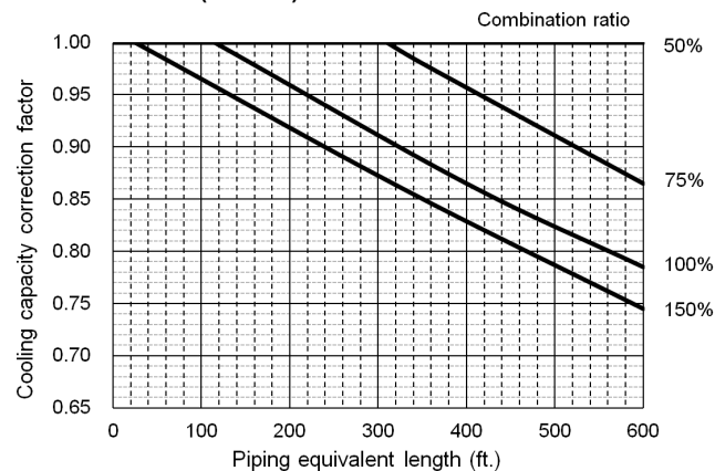
38VMA192RDS5-1(RDS6-1)
