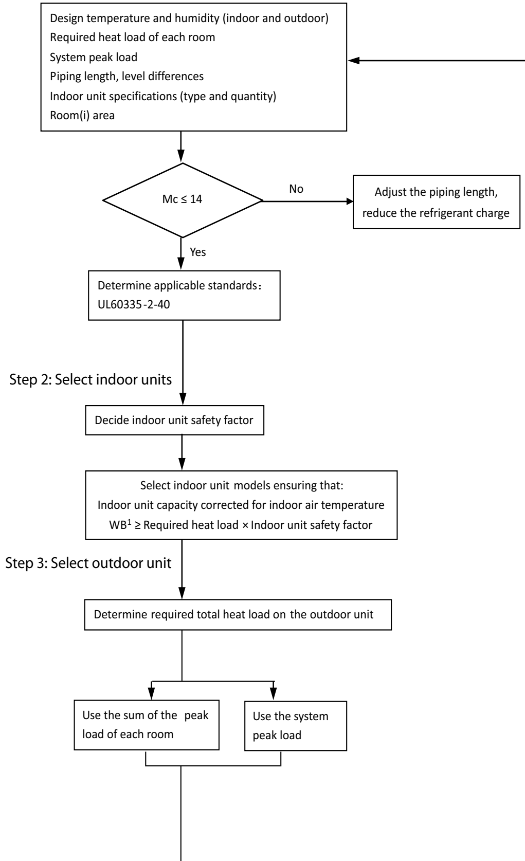
Fig. 5 —Selection Procedure
