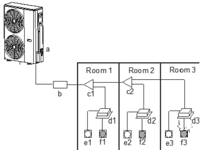
Fig. 30 —Potential Refrigerant Leak Scenario
