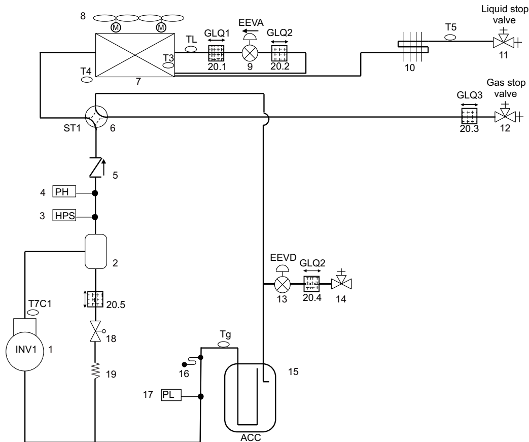
Fig. 13 —4.0/5.0 ton piping diagram
