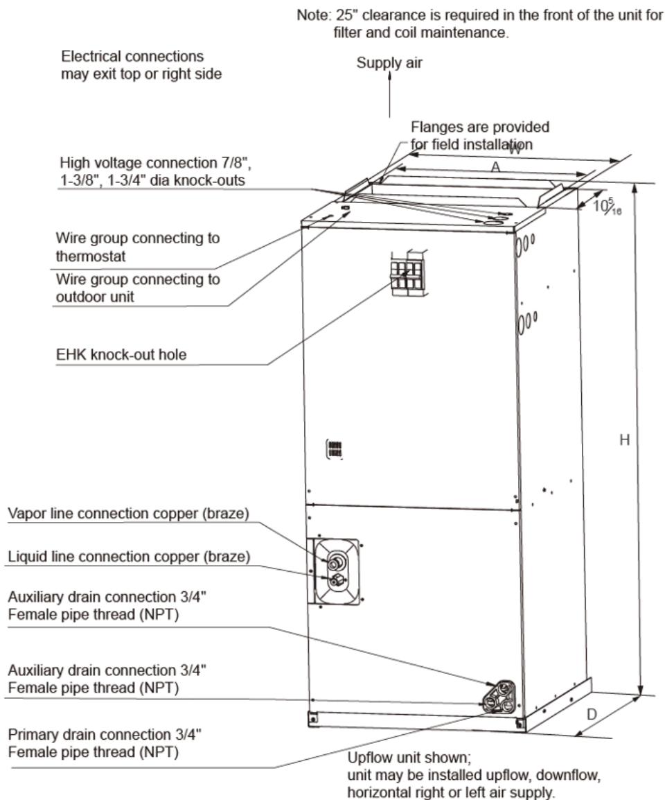
Fig. 2 —Dimensions - All Sizes
