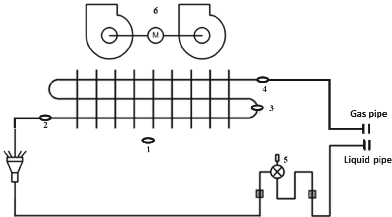
Fig. 5 —Piping Diagram
