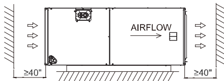
Fig. 3 —Clearances in the Horizontal Position
