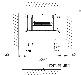
Fig. 4 —Clearances in the Vertical Position
