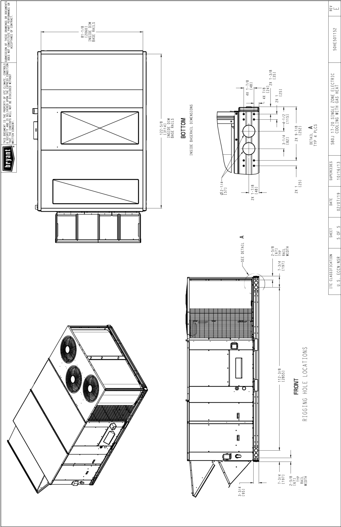
580J*18 BOTTOM VIEW
