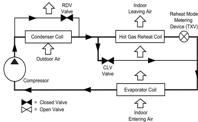
Subcooling Mode (Reheat1) — Perfect Humidity System with Single Stage Cooling
