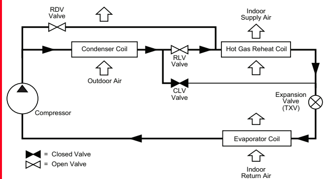
Hot Gas Reheat Mode (Reheat2) — Perfect Humidity System with 2-Stage Cooling
