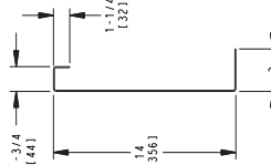
BASE RAIL CROSS SECTION TYP 2 SIDES
