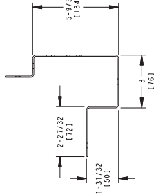
BASE RAIL CROSS SECTION TYP 2 SIDES
