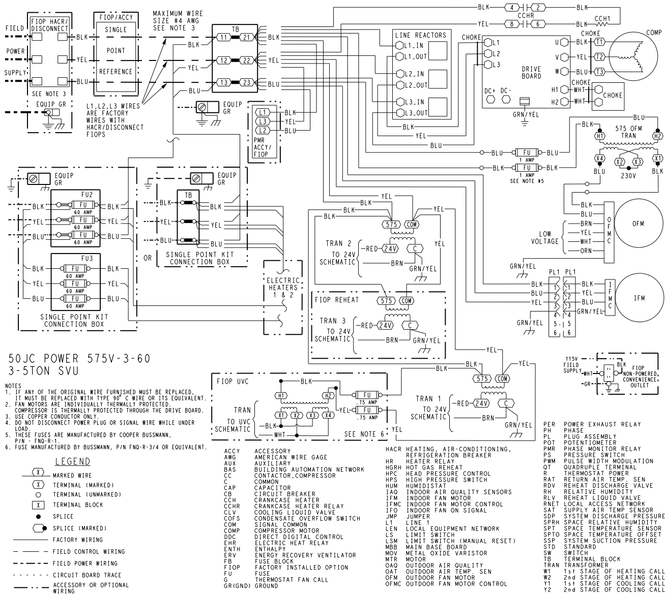
Typical Power Wiring Diagram — 50JC 04-06, 575/3/60 Unit Shown
