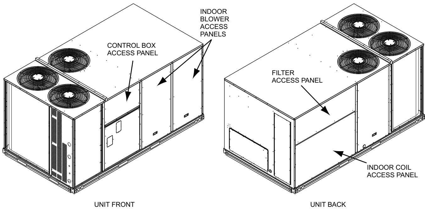
Fig. 8 — 50FCQ 14 Panel and Filter Locations
