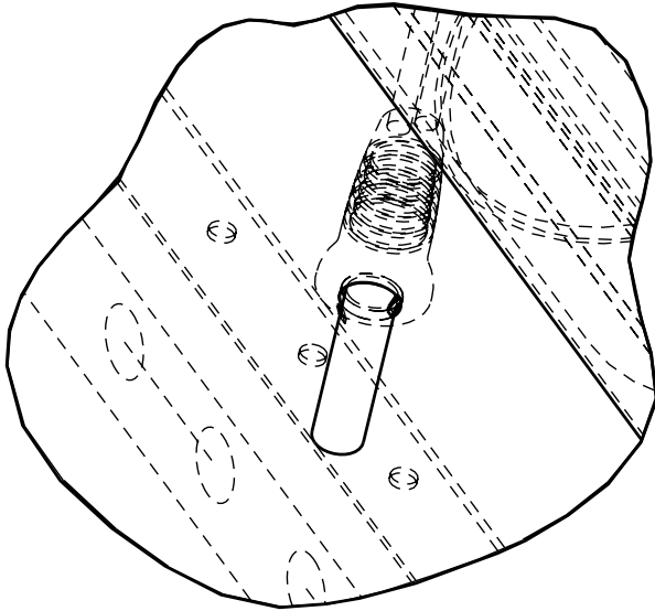
Fig. 15 — SAT and OAT Thermistor Mounting
