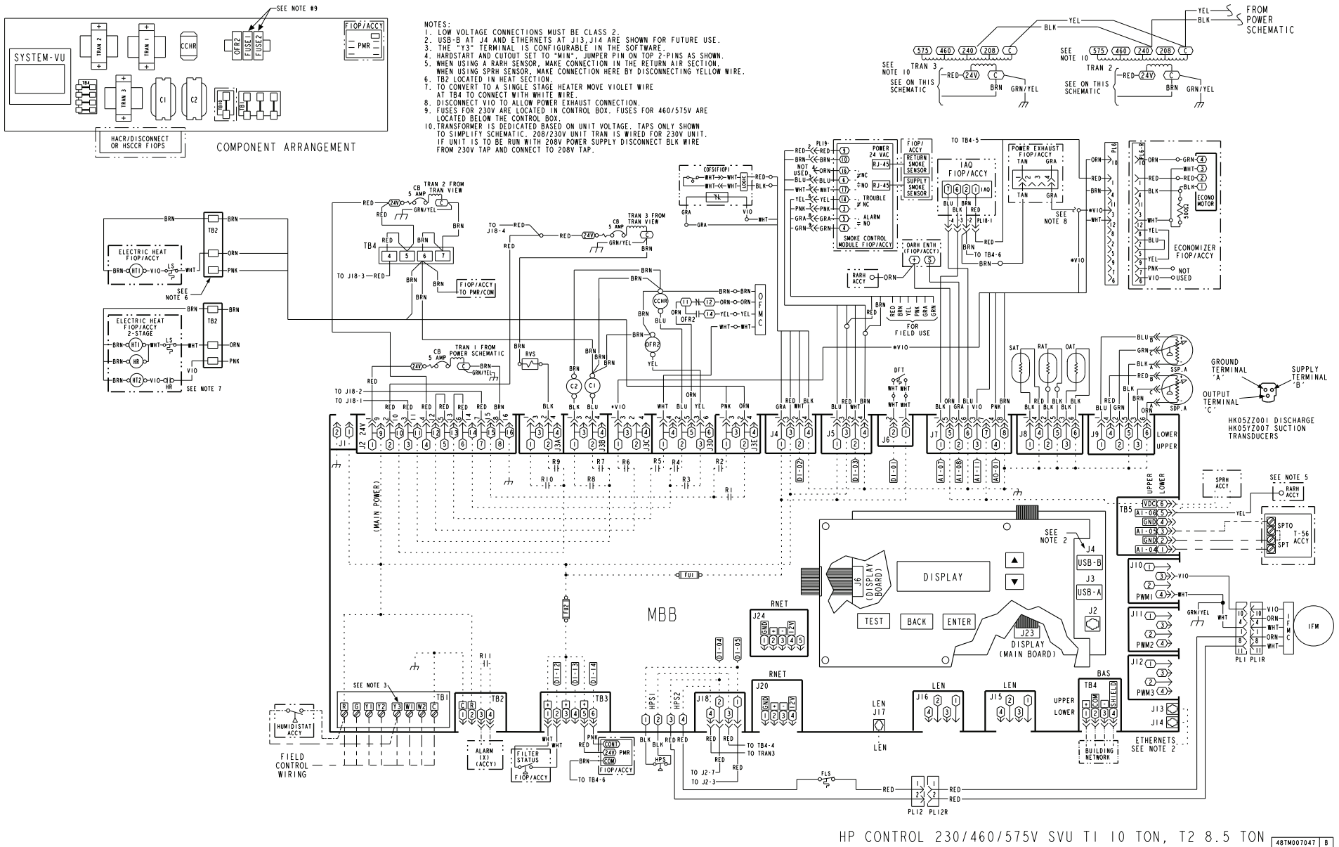
Fig. 19 — 50FCQ12 SystemVu Control Schematic
