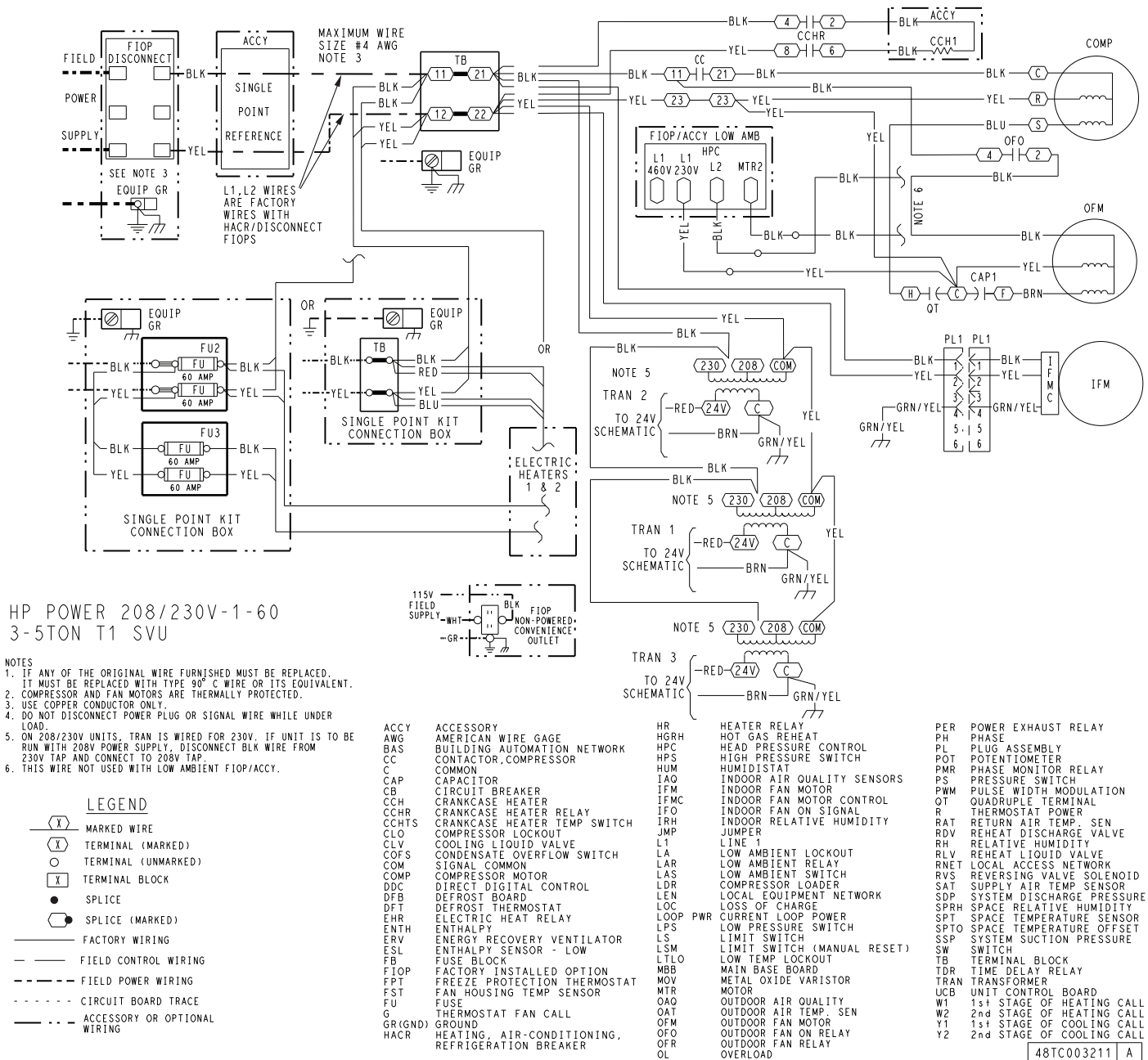
Fig. 22 — Typical Single Phase 230V SystemVu Power Schematic (50FCQ 04-06 shown)
