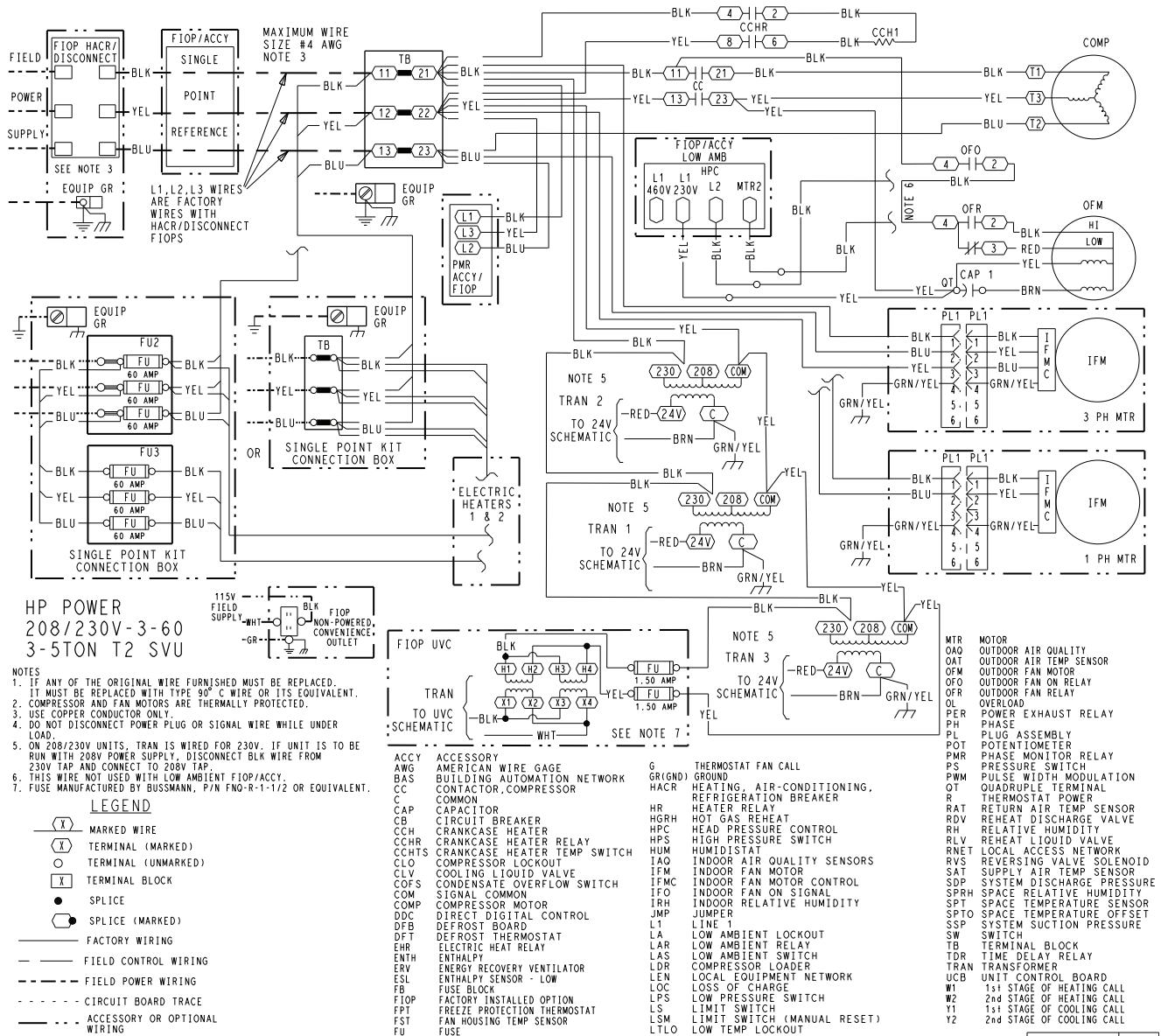
Fig. 24 — Typical 50GCQ 04-06 SystemVu Power Schematic (208/230V-3-60 shown)
