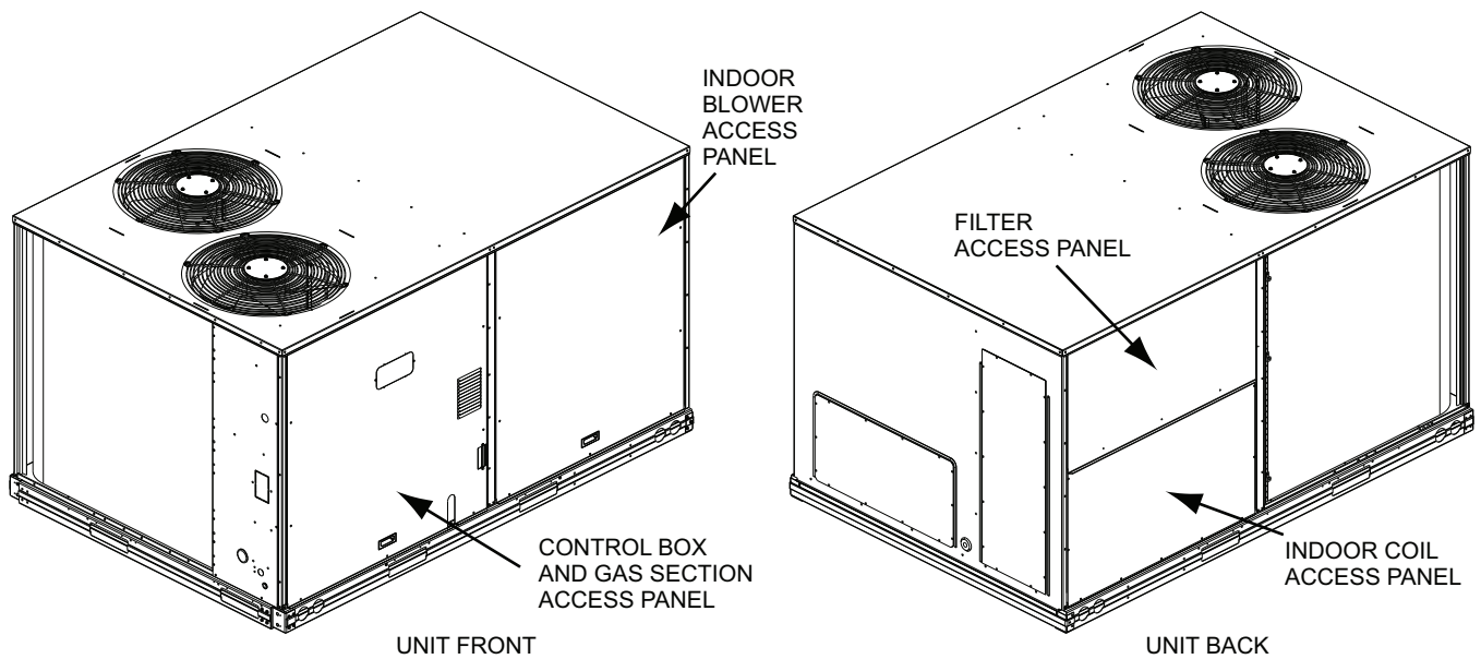
Fig. 7 — 50FCQ 08-12 Panel and Filter Locations
