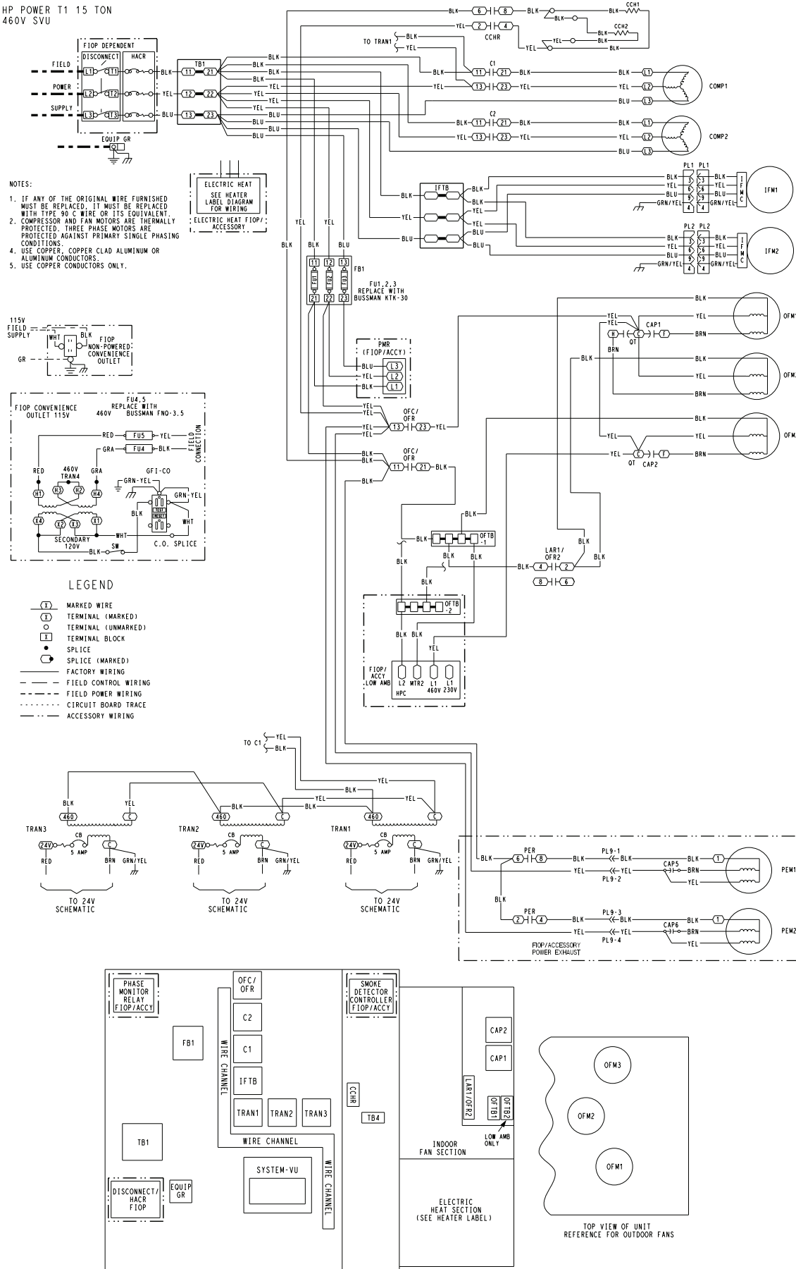
Fig. 28 — Typical 50FCQ17 SystemVu Power Schematic (460v shown)
