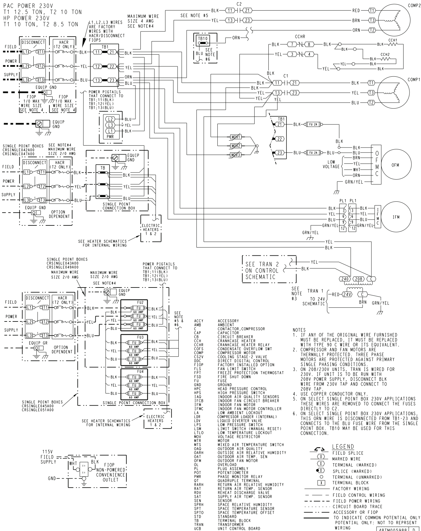
Fig. 26 — Typical 50FCQ12 SystemVu Power Schematic (230v shown)
