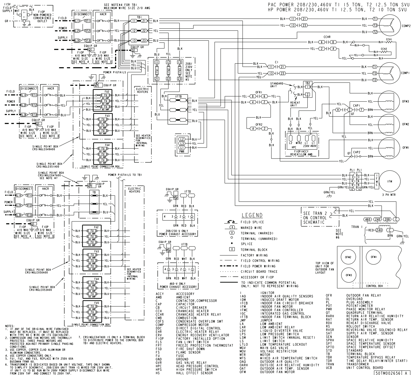
Fig. 27 — Typical 50FCQ14 SystemVu Power Schematic
