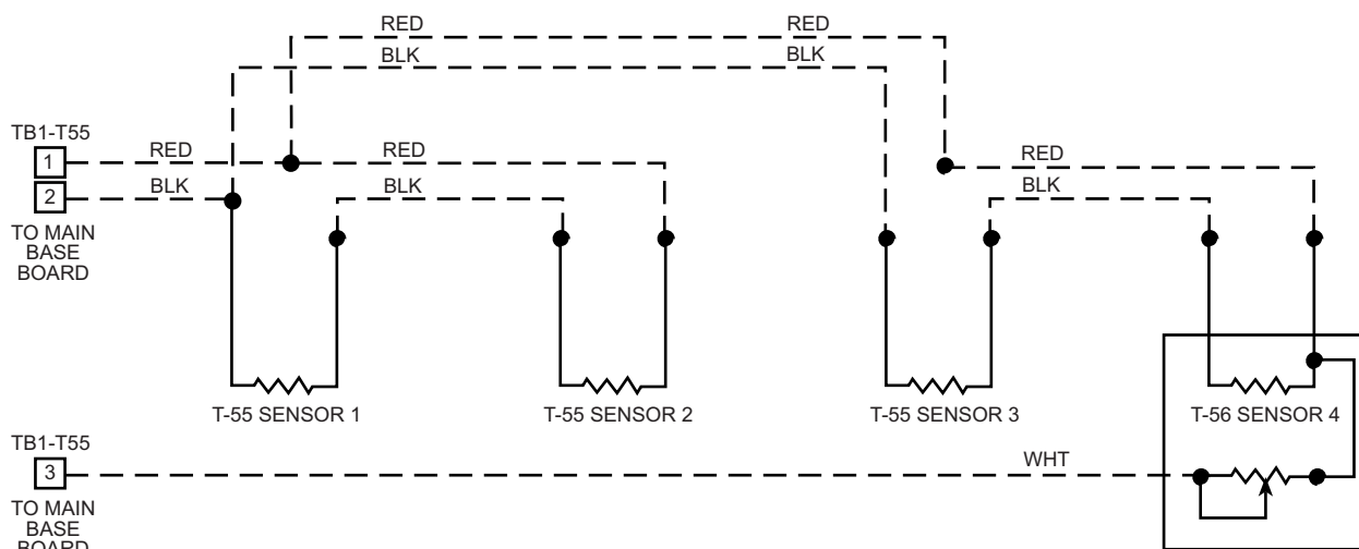
Fig. 32 — Space Temperature Sensor Averaging with 3 T-55 Sensors and One T-56 Sensor
