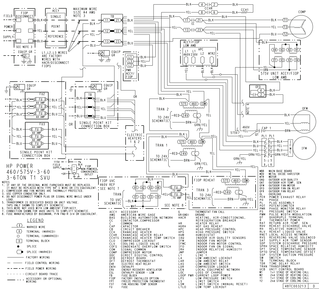
Fig. 23 — Typical 50FCQ 04-07 SystemVu Power Schematic (460/575V-3-60 shown)
