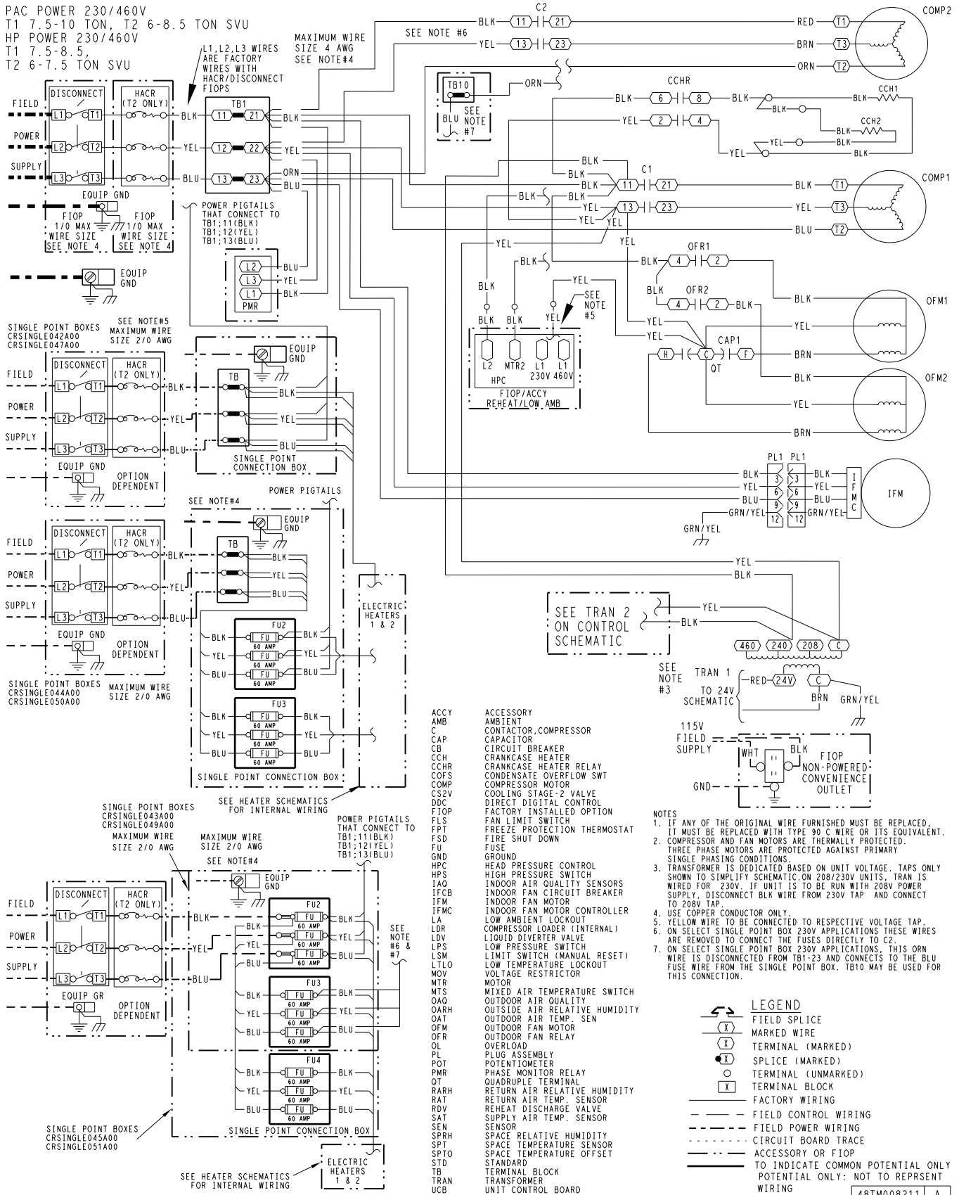
Fig. 25 — Typical 50FCQ08-09 SystemVu Power Schematic (230/460v shown)
