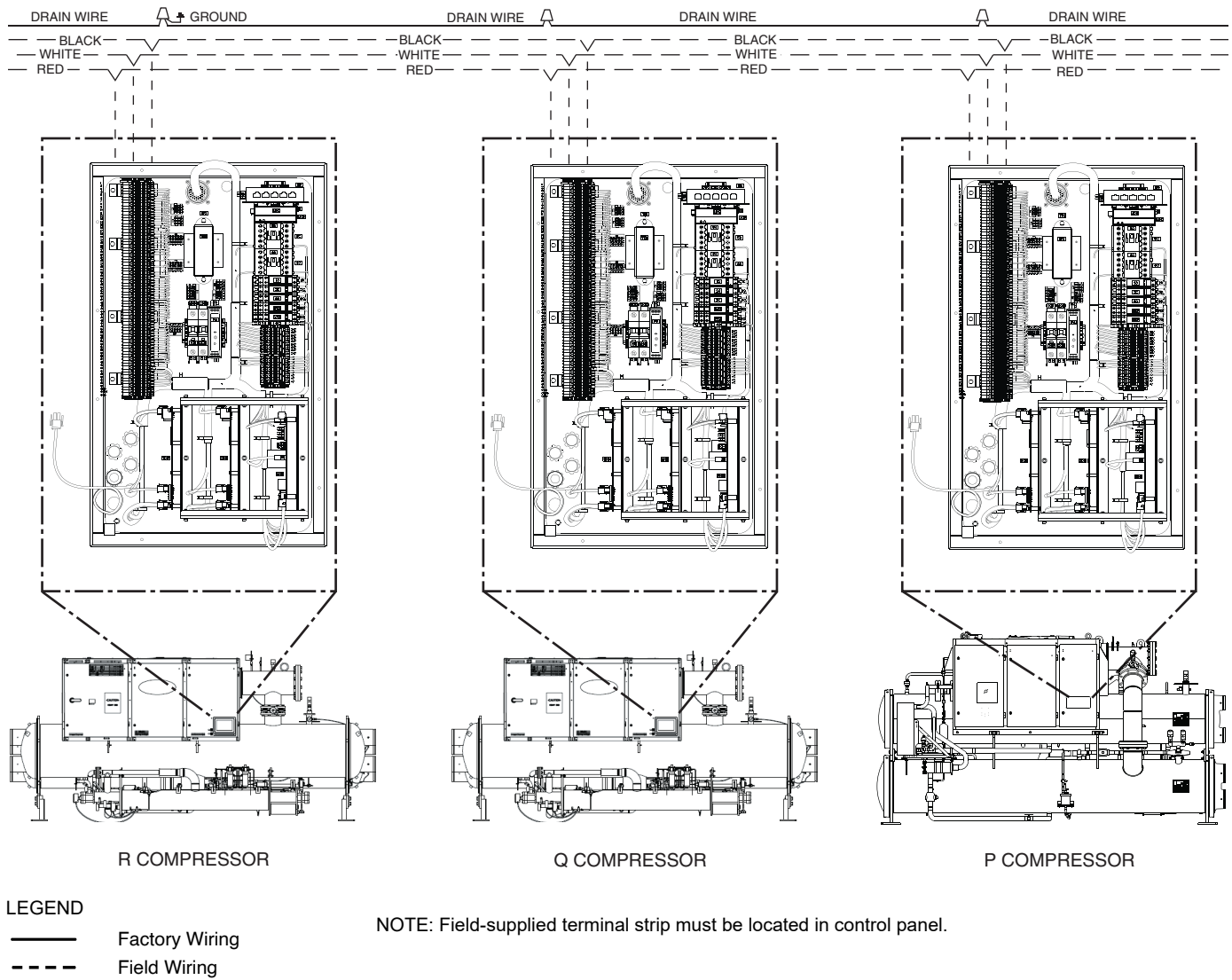
Fig. 63 — CCM Communication Wiring for Multiple Chillers (Typical)
