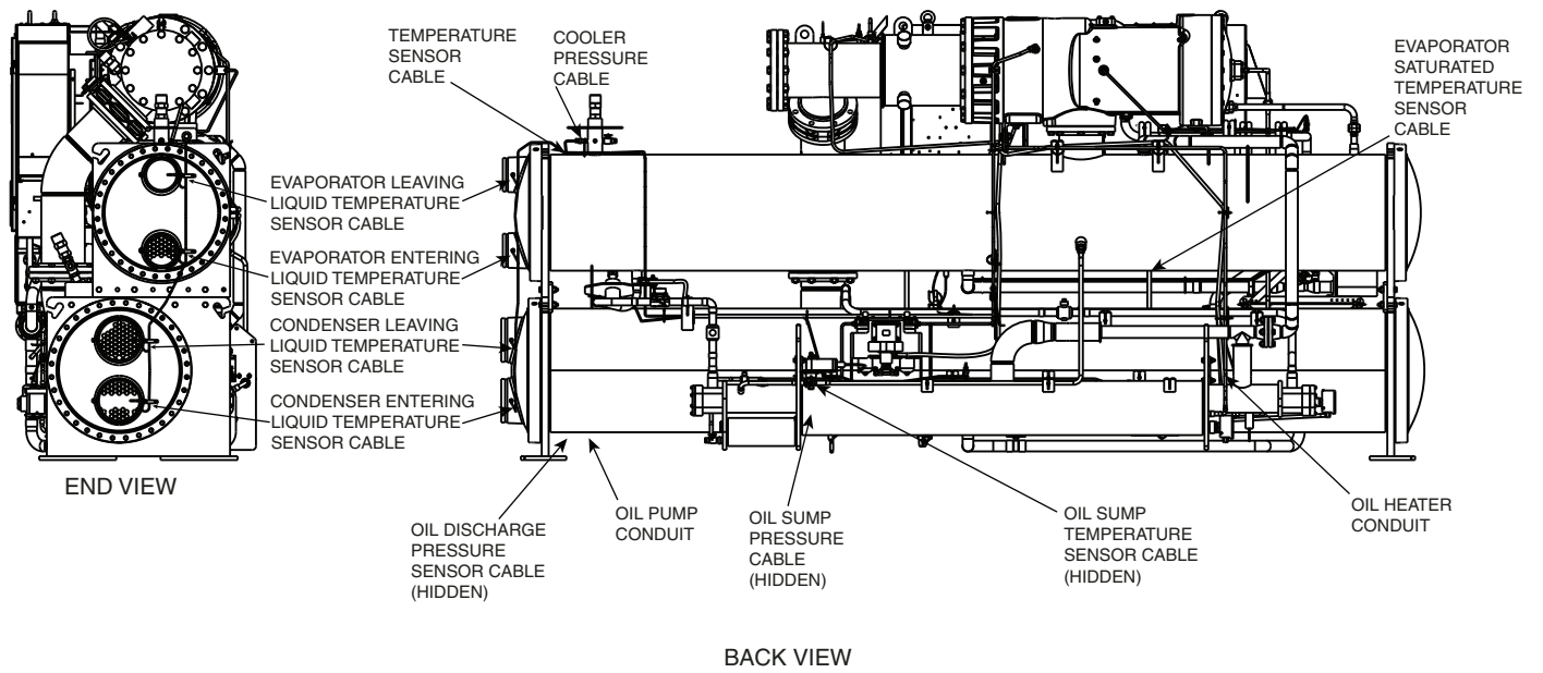
Fig. 17 — Electrical Cable Routing (Unit with P Compressor Shown)
