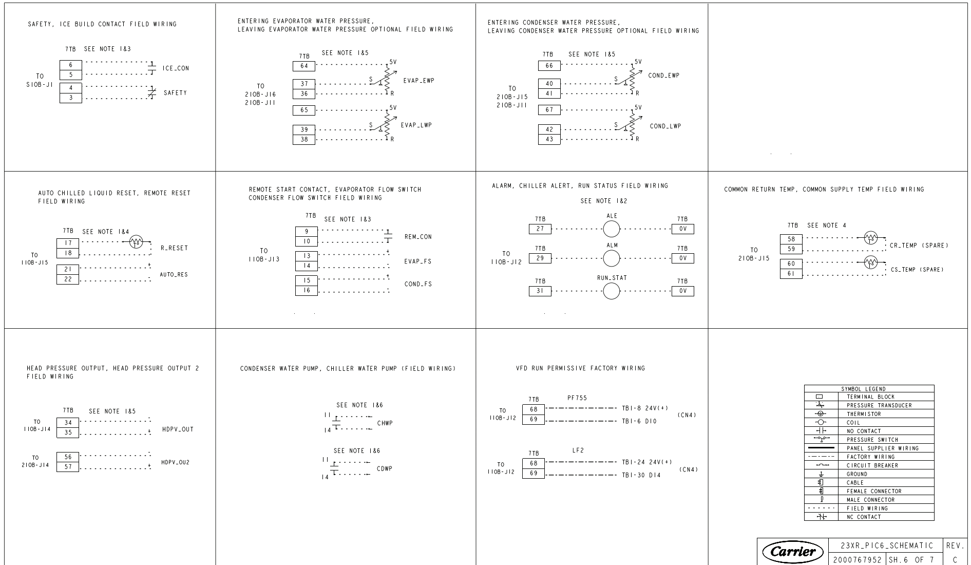
Fig. 58 — 23XRV Controls Schematic (cont)
