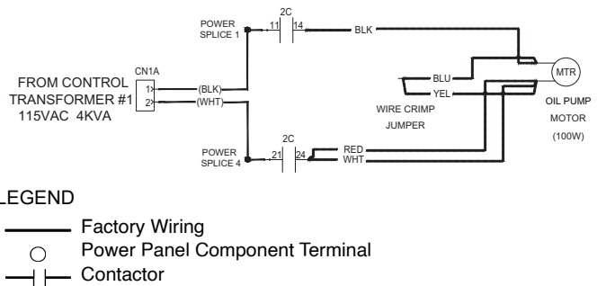
Fig. 65 — Oil Pump Wiring
