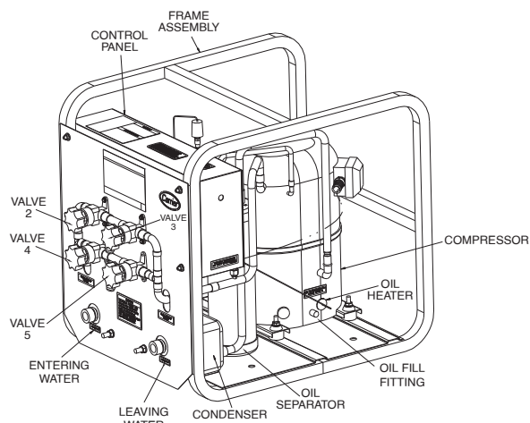
Fig. 54 — Pumpout Unit
