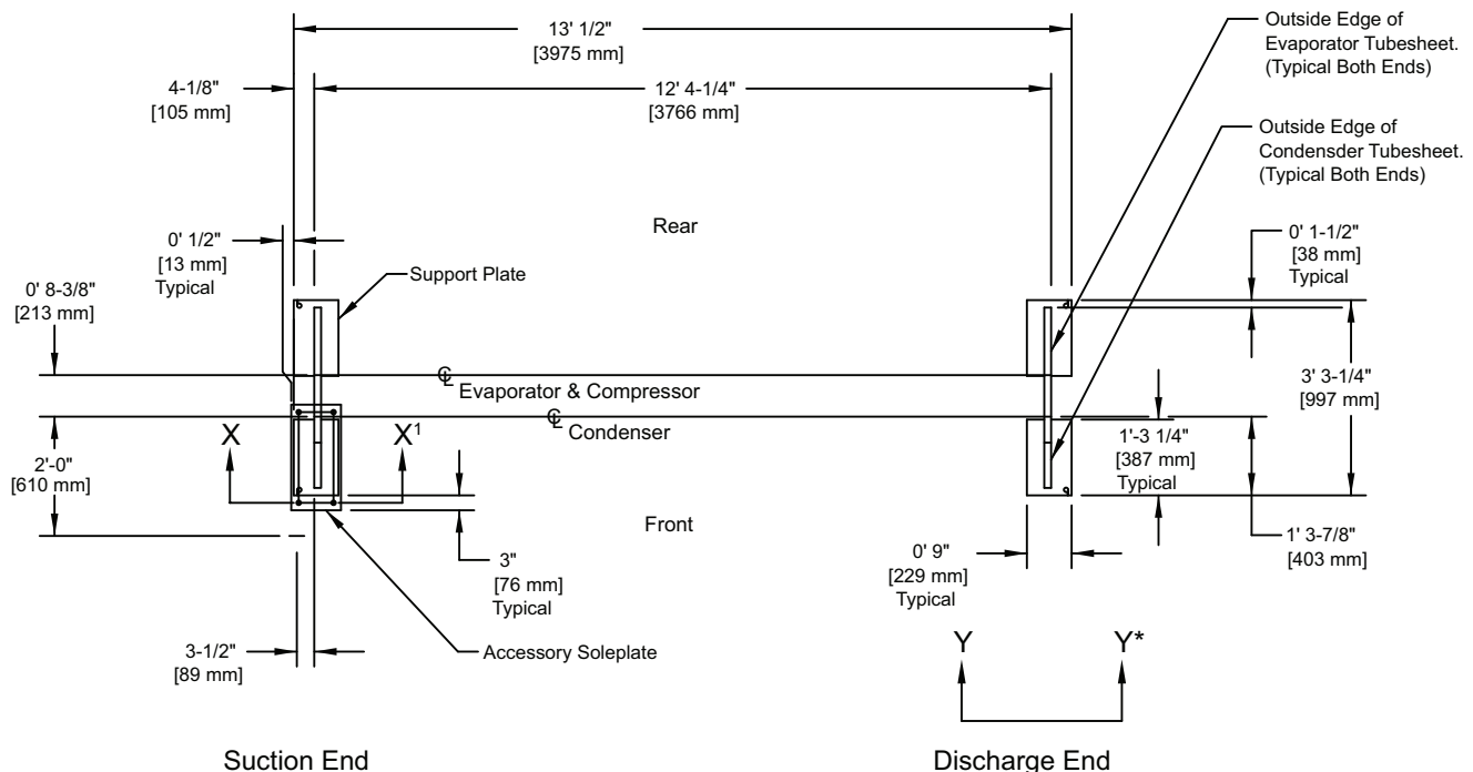
Fig. 40 — 23XRV30-57 Machine Footprint
