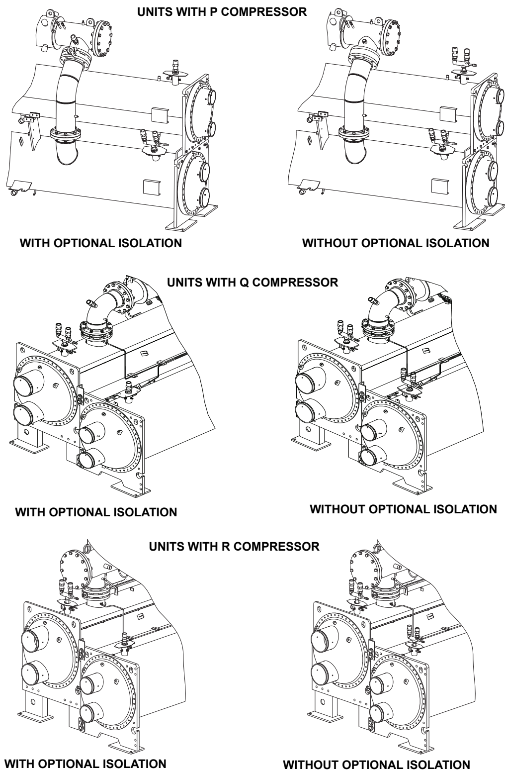
Fig. 55 — Relief Valve Arrangements
