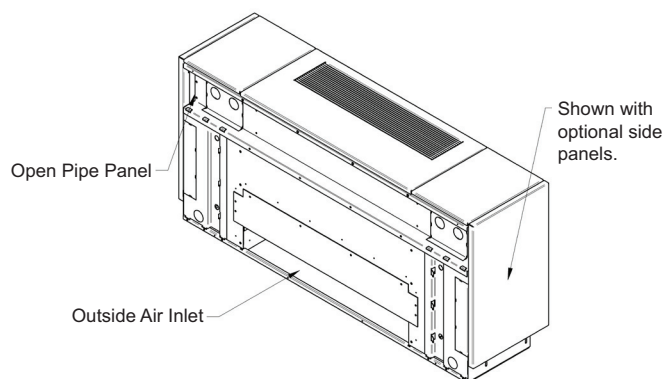
Rear Outside Air — Open Pipe Tunnel
