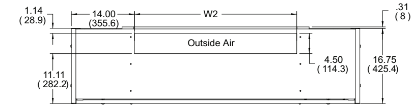
REAR VIEW
