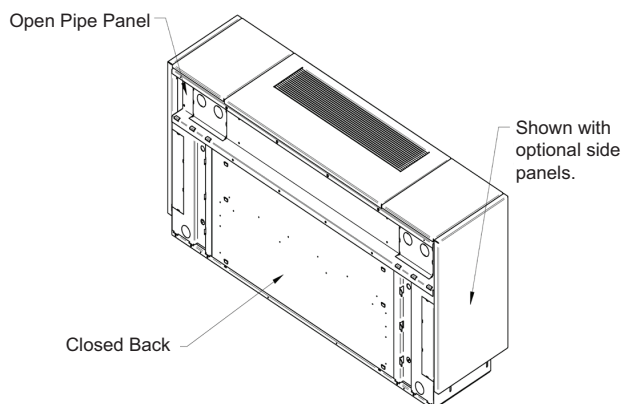
No Outside Air — Open Pipe Tunnel
