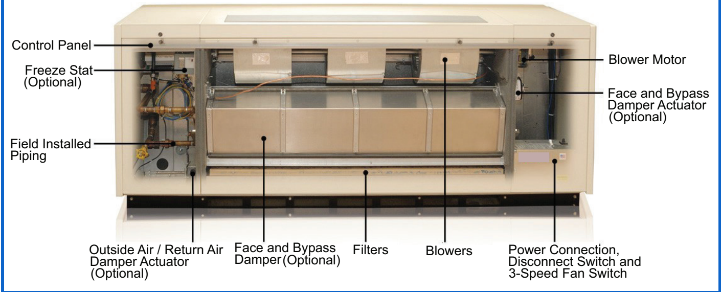
Component Layout
