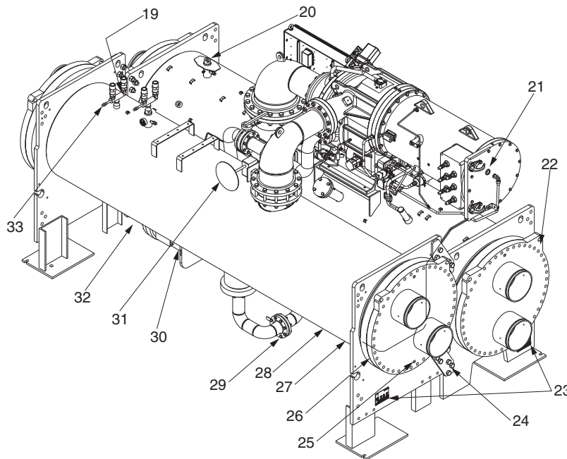
REAR VIEW
