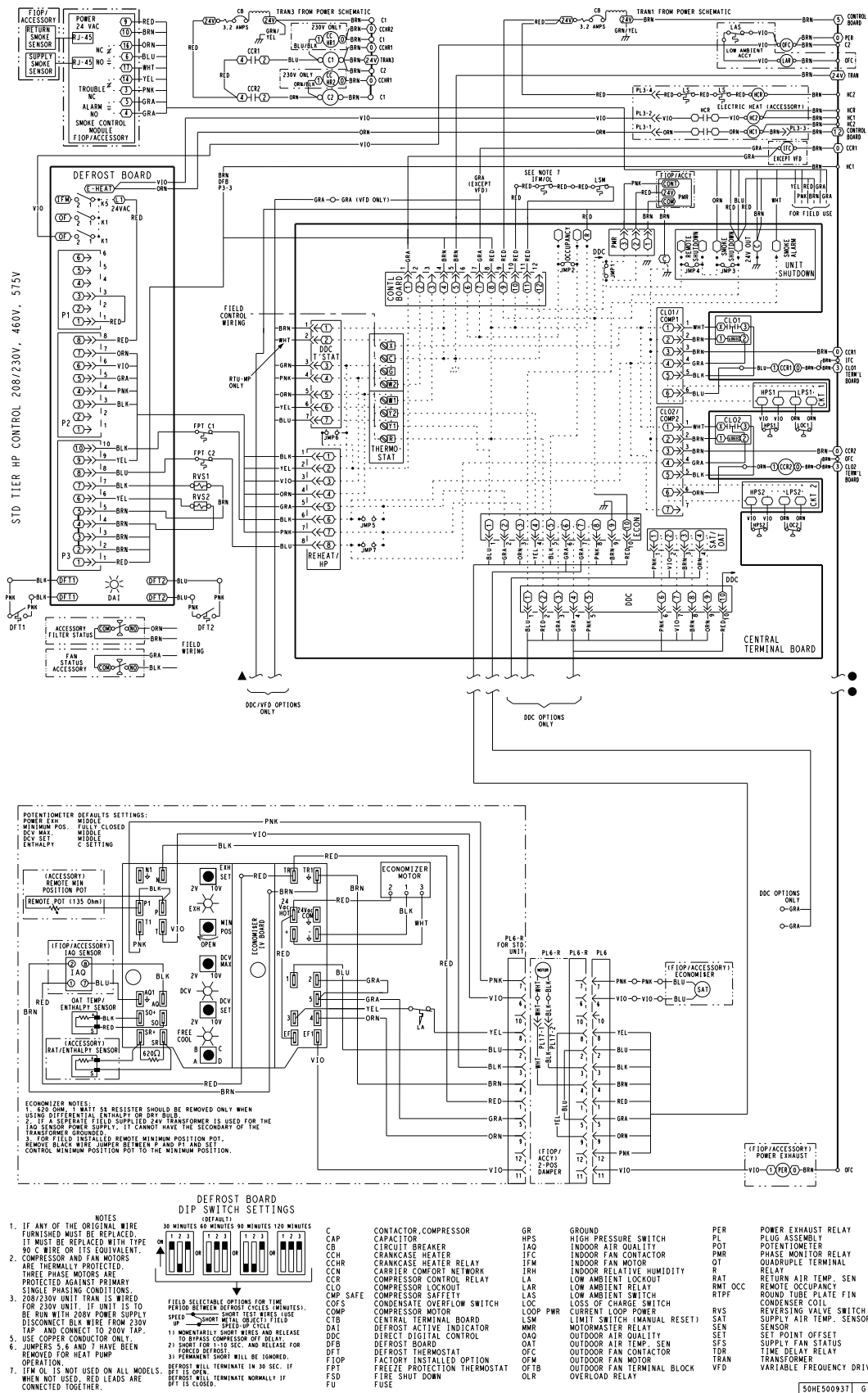
TYPICAL CONTROL DIAGRAM
