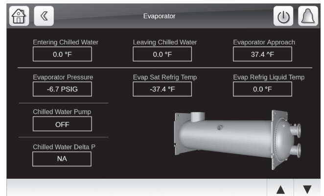
Fig. 25 — Evaporator Status
