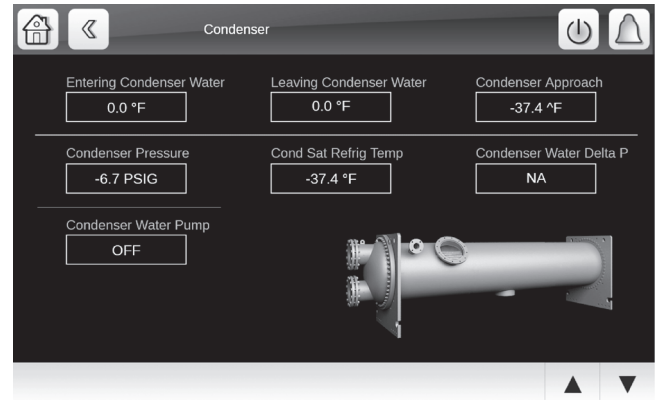
Fig. 24 — Condenser Status
