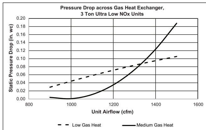
Pressure Drop across Gas Heat Exchanger, 48FE Ultra Low NOx — 3 Ton Units
