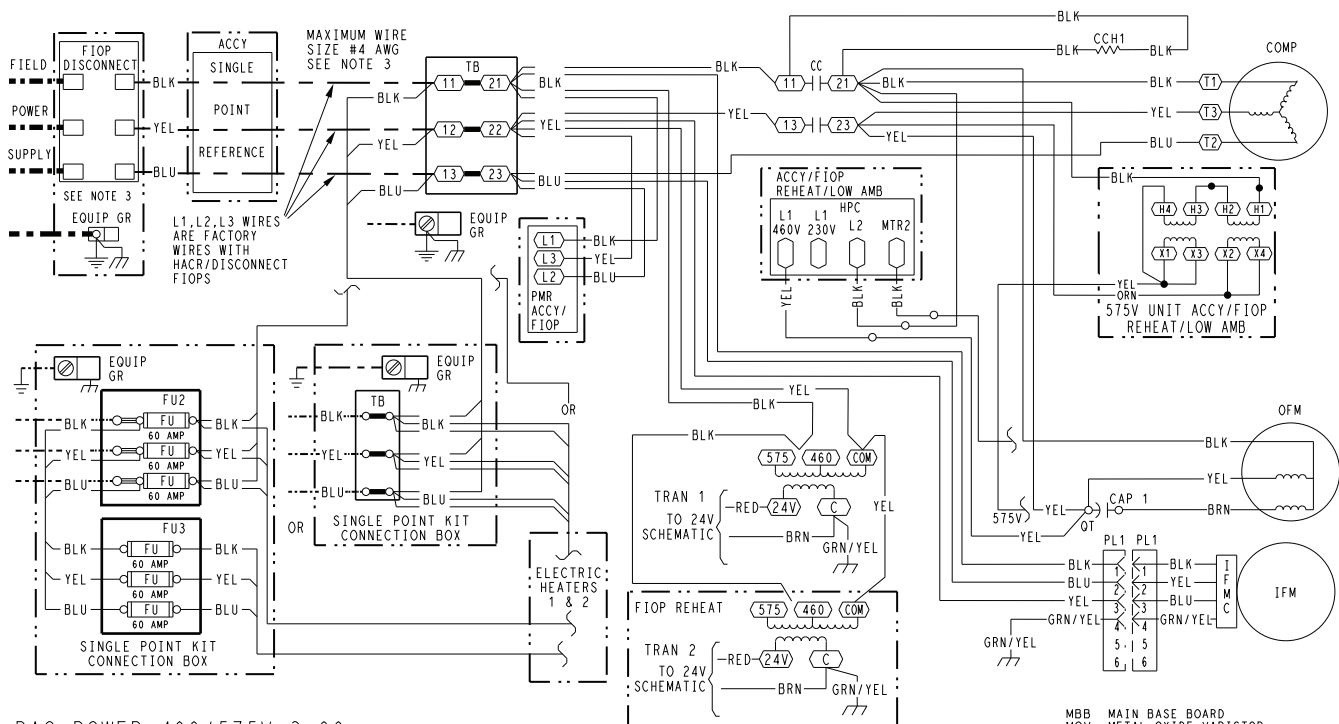
Typical 50FE 04-07 Power Wiring Diagram, 460/575-v Unit Shown
