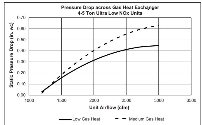
Pressure Drop across Gas Heat Exchanger, 48FE Ultra Low NOx — 4 to 5 Ton Units
