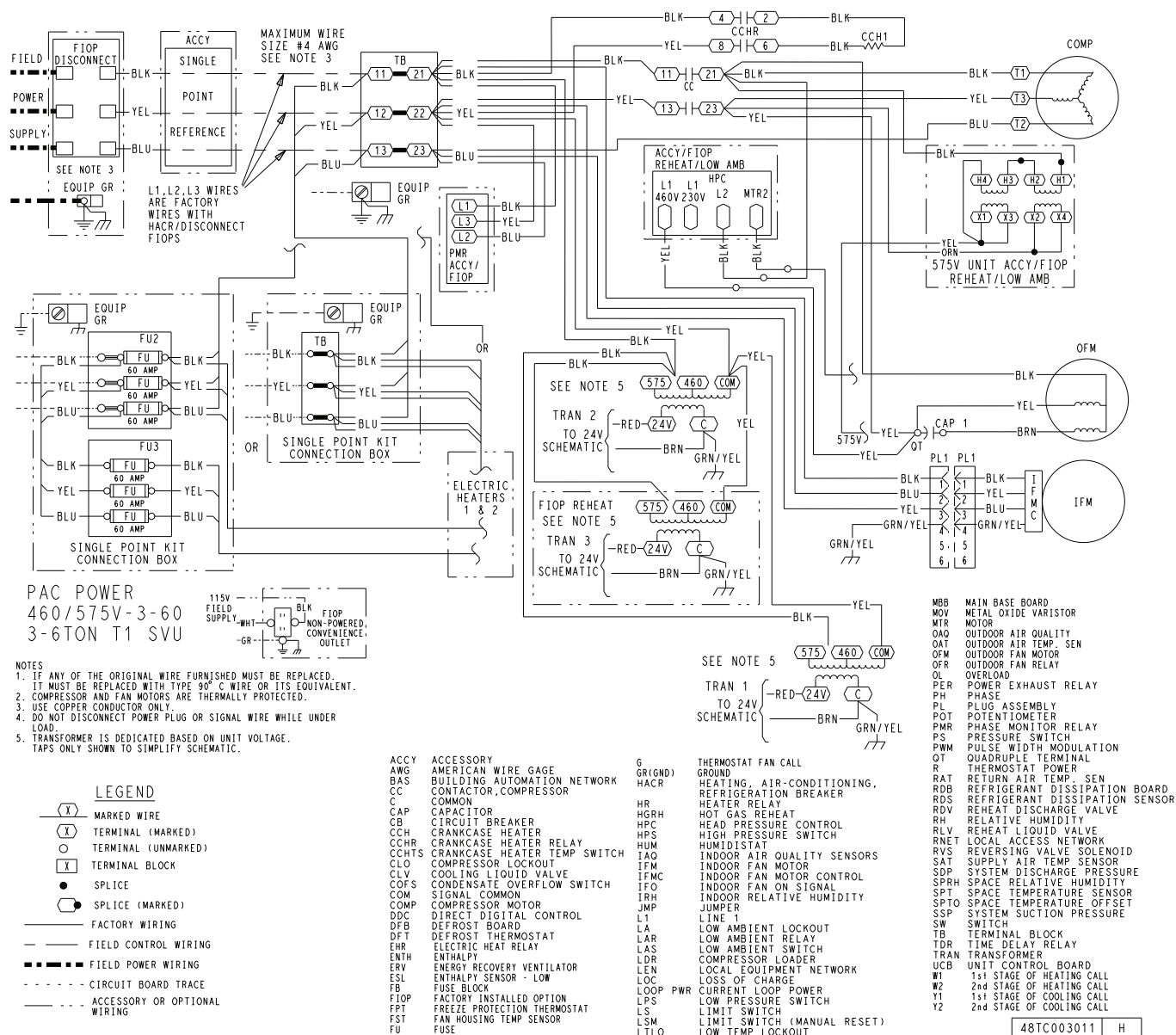
Typical Power Wiring Diagram for SystemVu™ Controller Units, 50FE 04-07, 460/575-3-60 Units Shown
