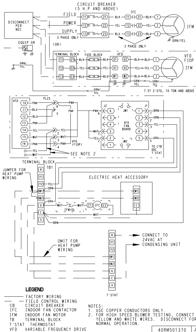
Fig. 37 — Typical Wiring Diagram — Split System Air-Handling Unit (524J with ACH550 VFD shown)
