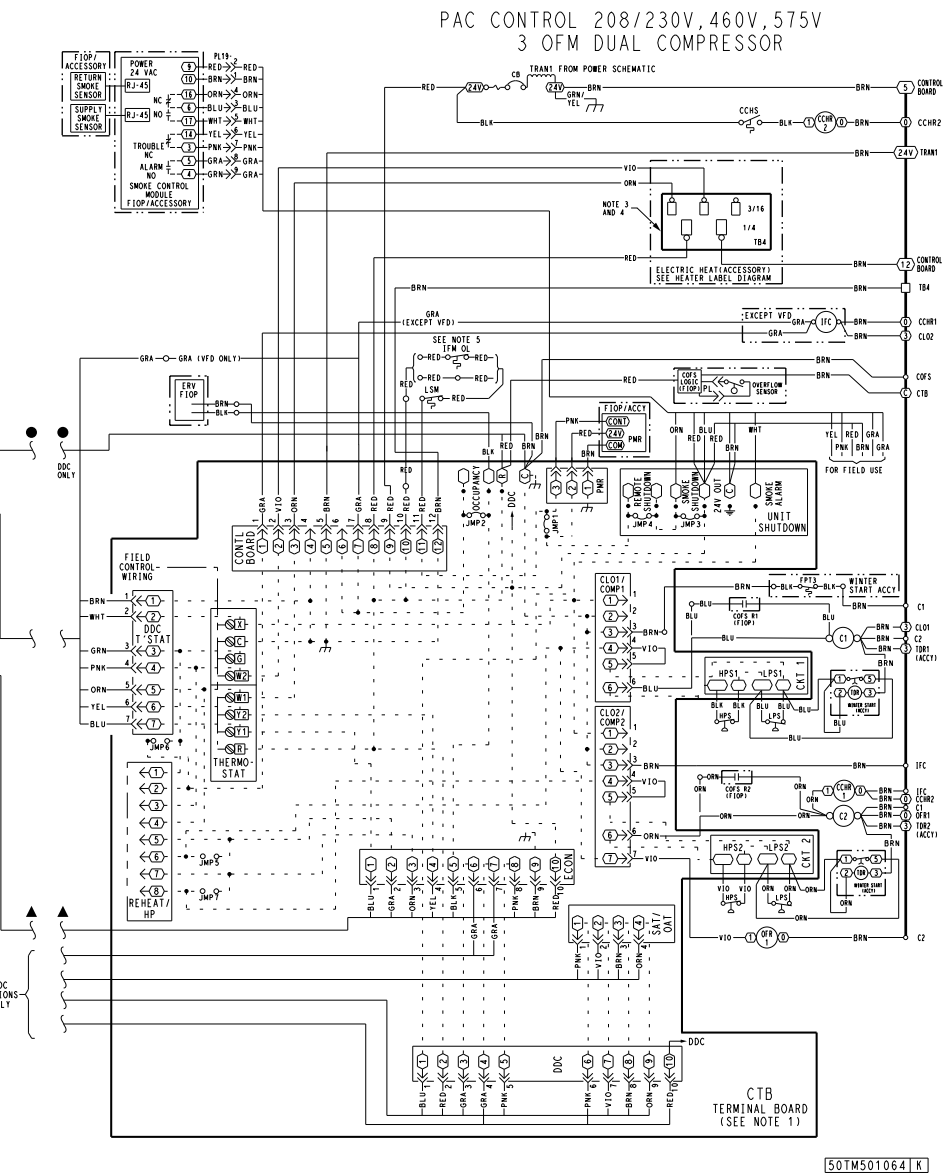
Fig. 34 — Typical Wiring Diagram — Single Package Rooftop Unit (551J*14 with ACH550 VFD shown)
