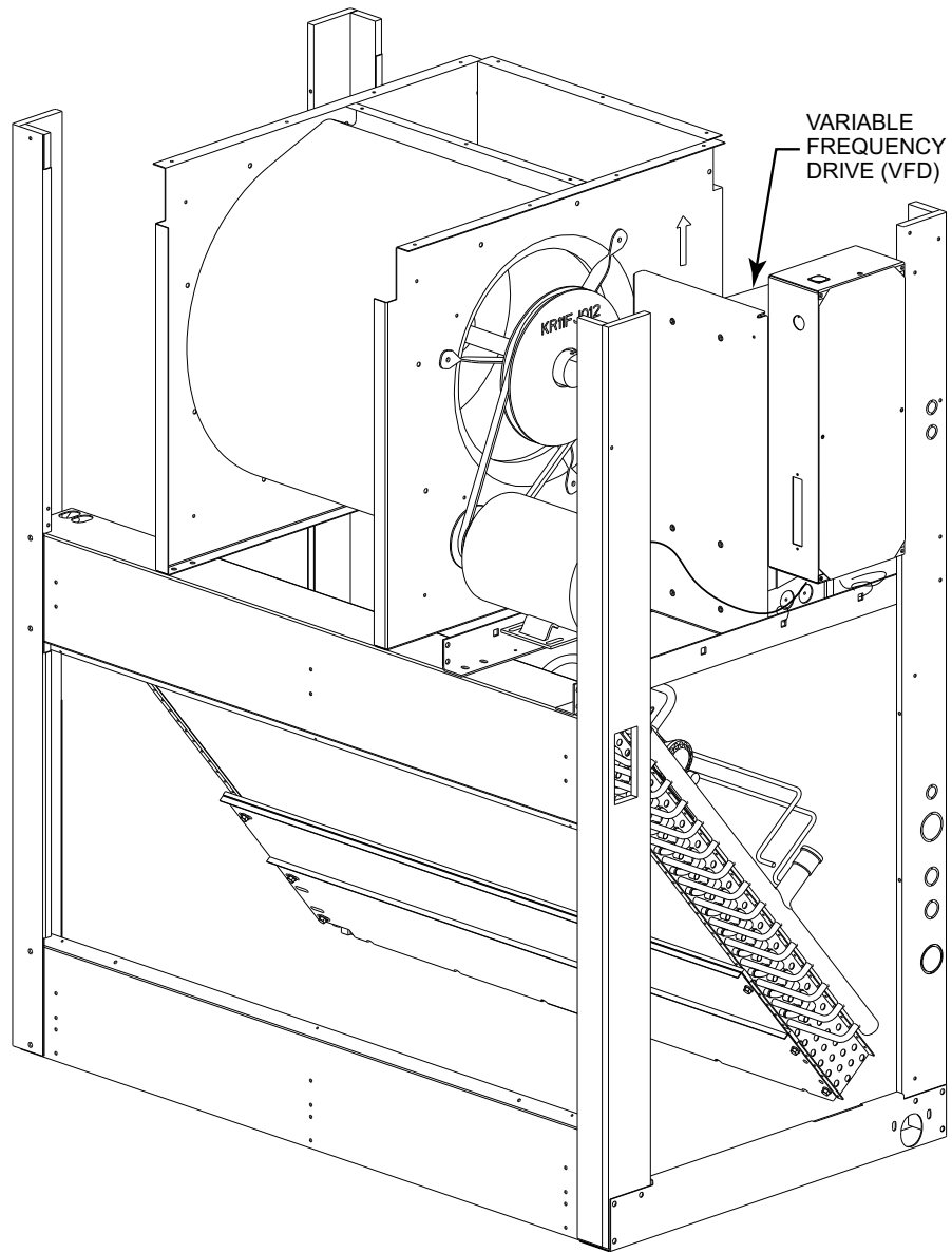
Fig. 20 — ACH550 VFD Location for the following units: 524J*07-12A and 524J*07-12H (575V only)
