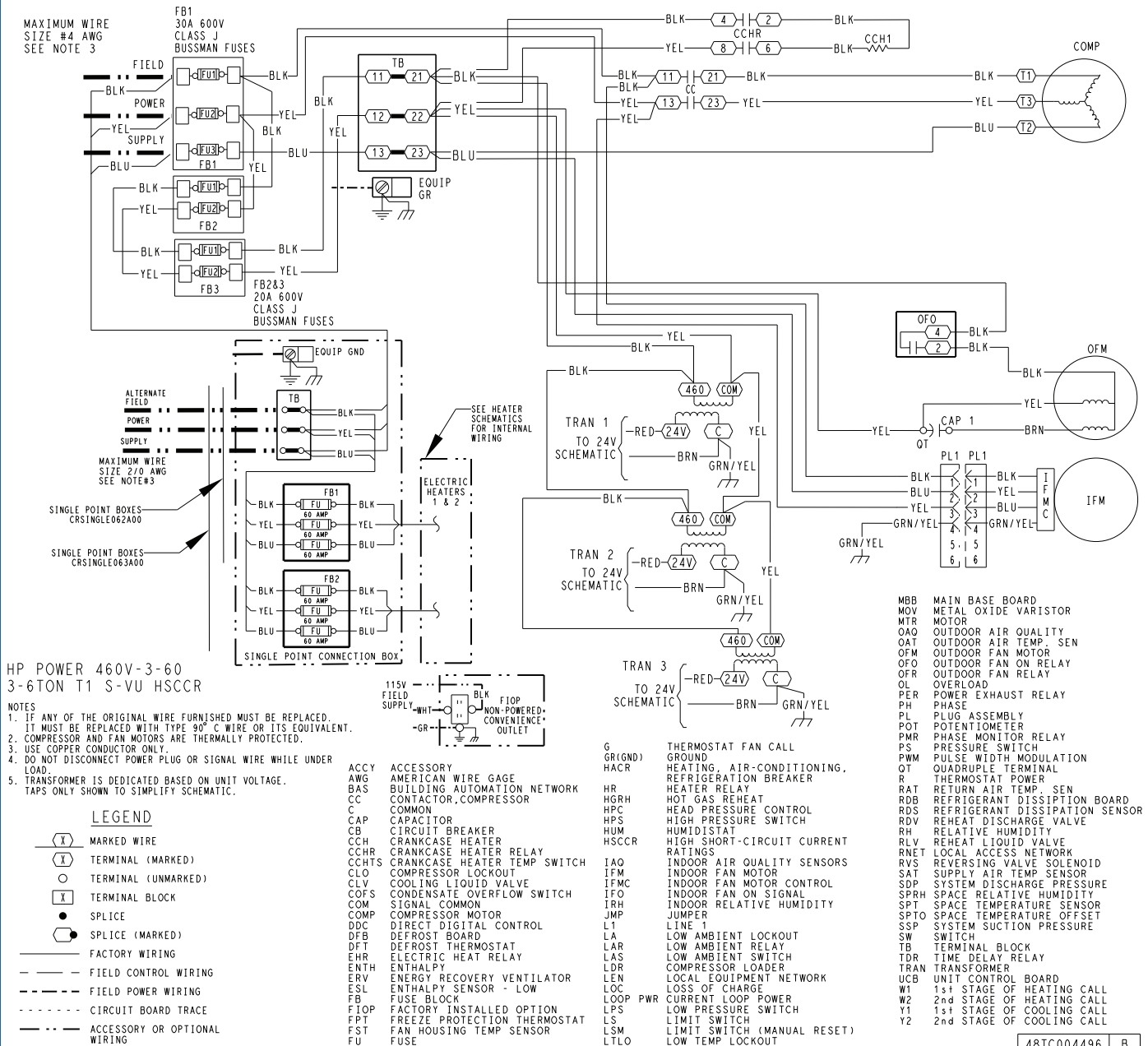
Typical 50FEQ 04-07 Power Wiring Diagram, SystemVu, 460-3-60 High SCCR Shown
