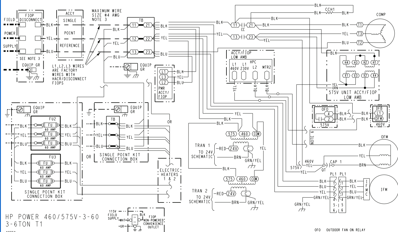
Typical 50FEQ 04-07 Power Wiring Diagram, Electromechanical, 460/575-3-60 Standard SCCR Shown
