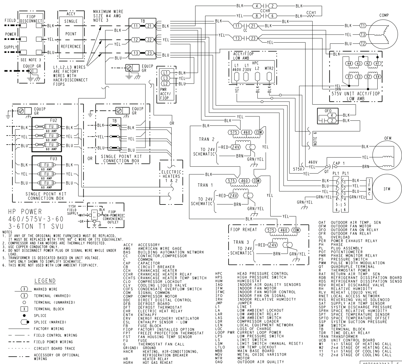
Typical 50FEQ 04-07 Power Wiring Diagram, SystemVu, 460/575-3-60 Standard SCCR Shown
