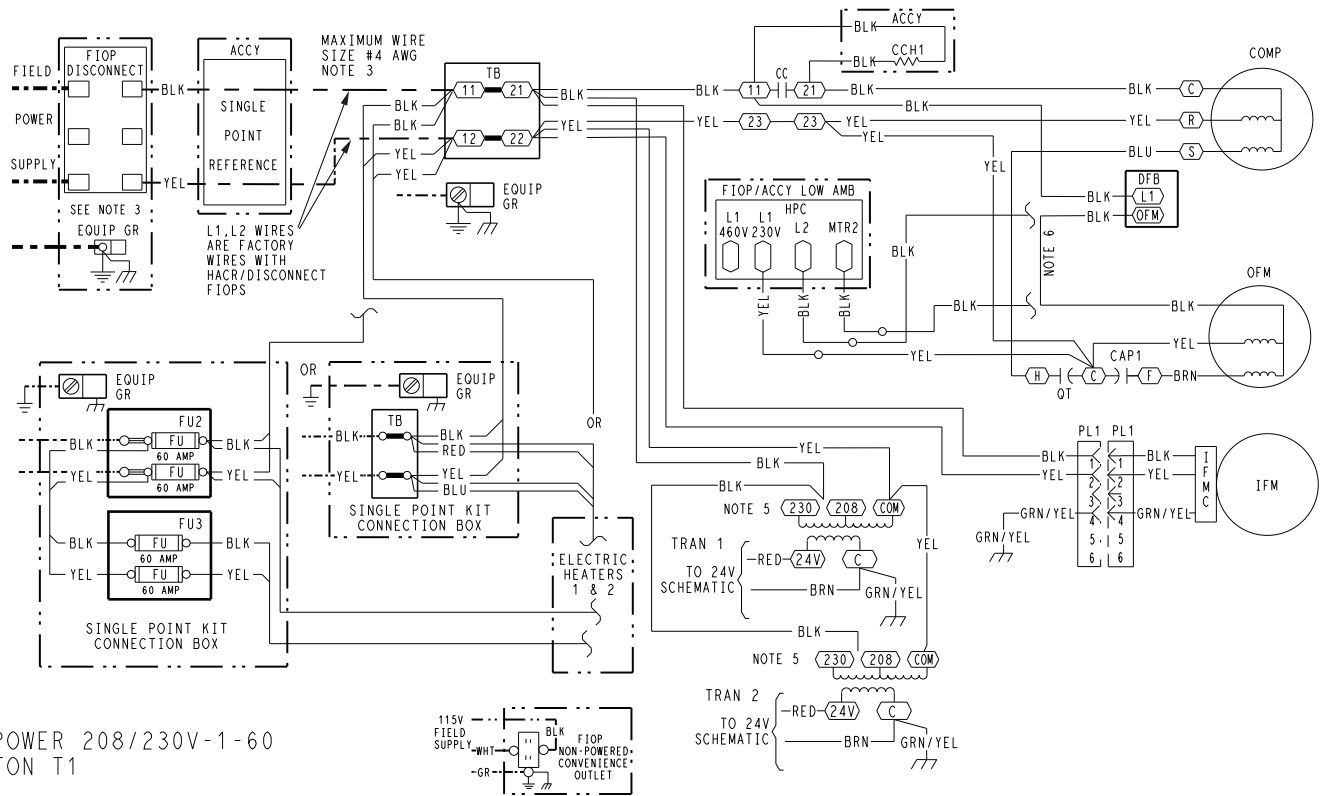
Typical 547K 04-06 Power Wiring Diagram, 208/230-1-60 Unit
