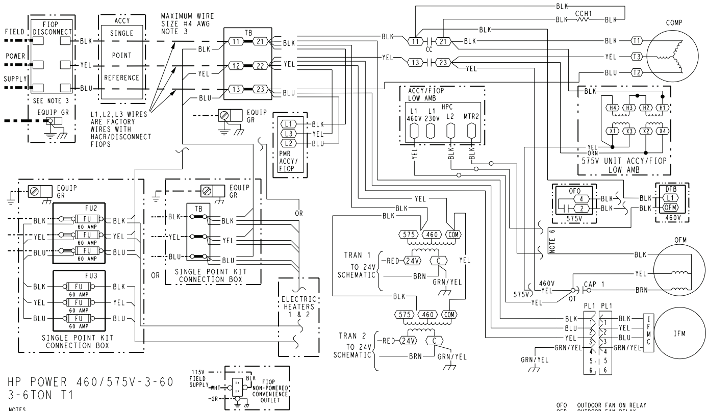
Typical 547K 04-07 Power Wiring Diagram, 460/575-3-60
