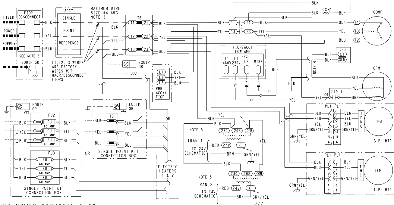
Typical 547K 04-07 Power Wiring Diagram, 208/230-3-60 Unit
