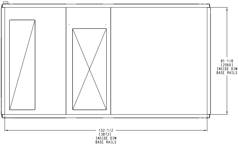
BOTTOM INSIDE BASERAIL DIMENSIONS
