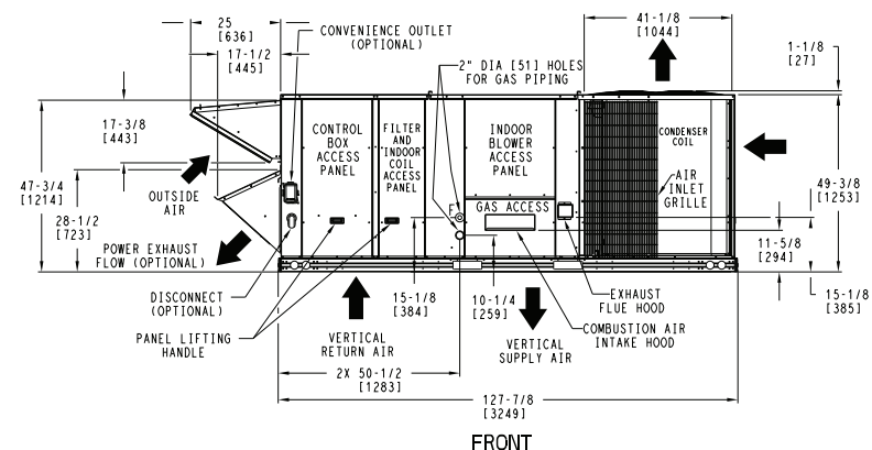
DEDICATED VERTICAL AIRFLOW UNIT 20 SIZE
