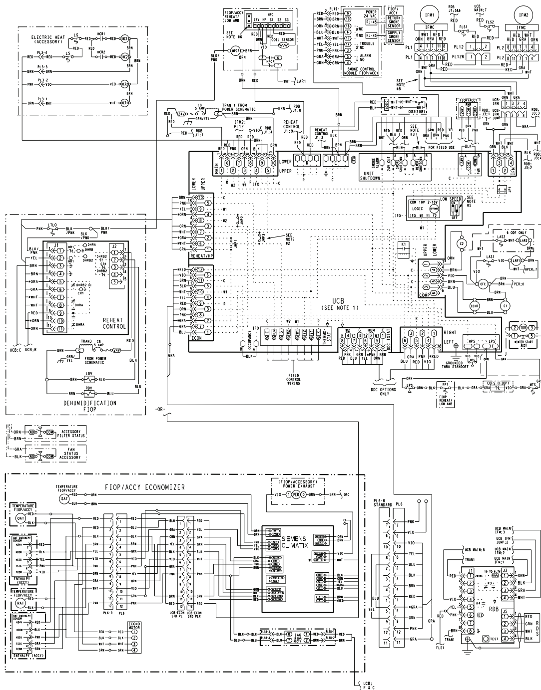
559L*20-30 Control Wiring Diagram, Electromechanical with POL224 Controller
