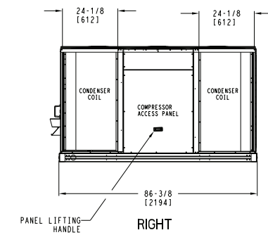
DEDICATED VERTICAL AIRFLOW UNIT 20 SIZE
