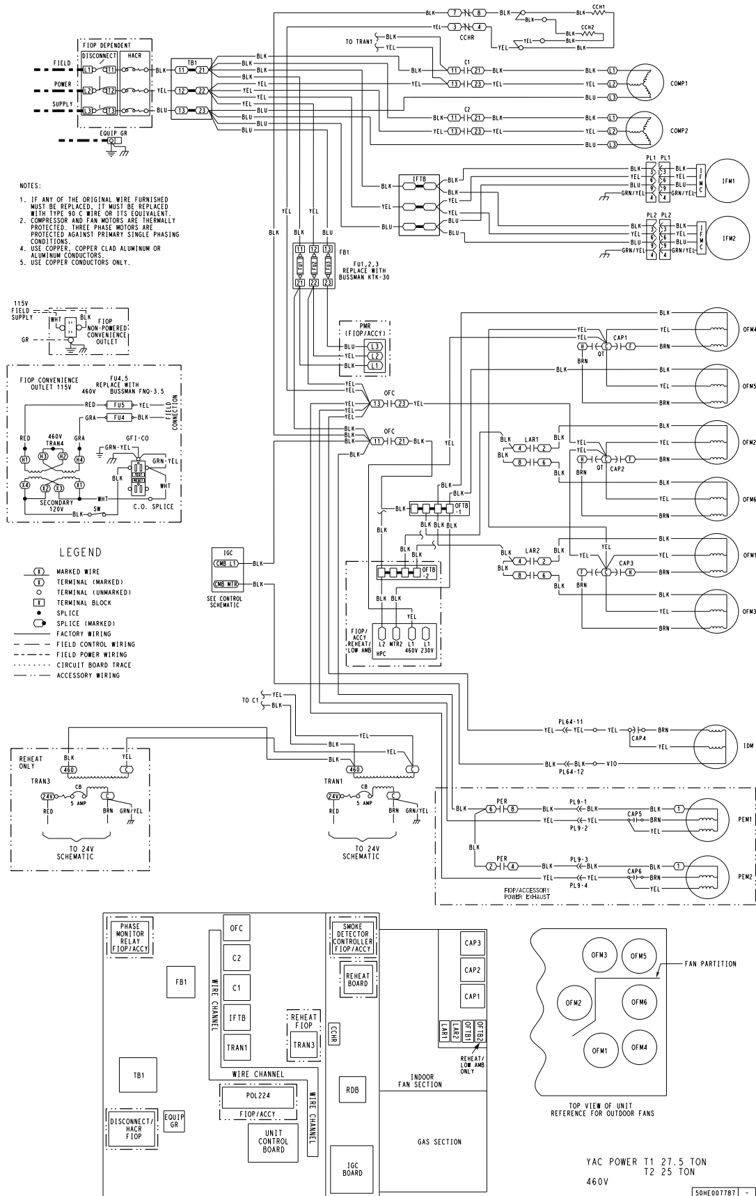
582L*30 Power Wiring Diagram, Electromechanical with POL224 Controller
