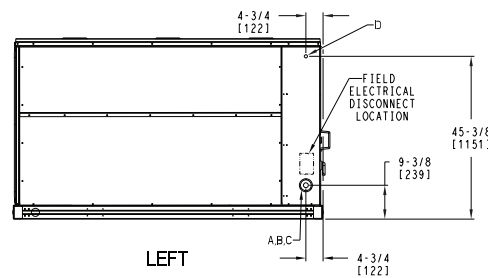
LEFT [ DEDICATED HORIZONTAL AIRFLOW UNIT RETURN AIRFLOW WITH ECONOMIZER ]
