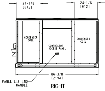
DEDICATED HORIZONTAL AIRFLOW UNIT 20 SIZE
