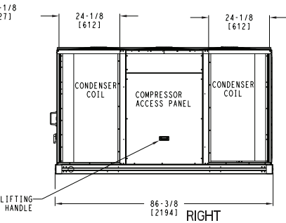
RIGHT DEDICATED HORIZONTAL AIRFLOW UNIT 20 SIZE
