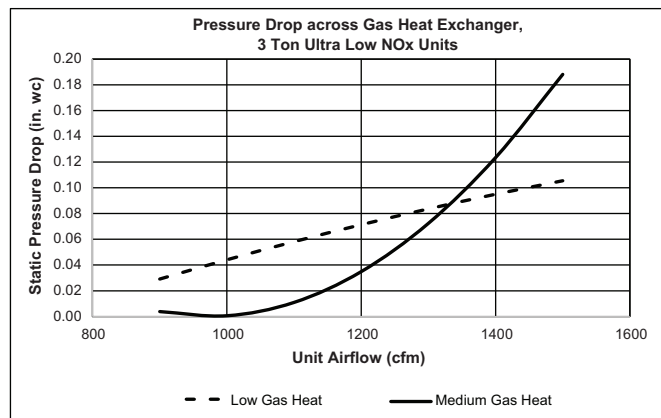
Pressure Drop across Gas Heat Exchanger, 582L Ultra Low NOx — 3 Ton Units
