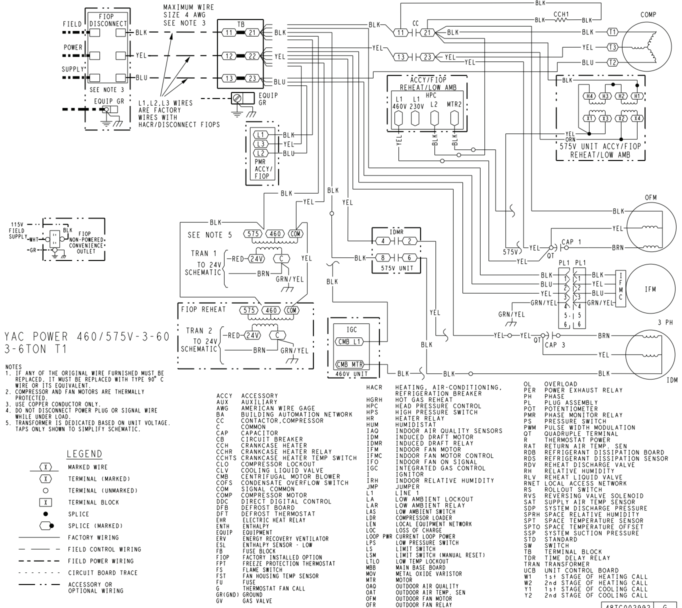
Typical Power Wiring Diagram for Electromechanical Units, 582L 04-07, 460/575-3-60 Units Shown
