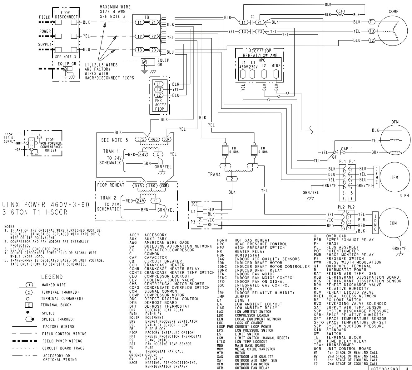
Typical Power Wiring Diagram for Electromechanical Units, 582L 04-06 Ultra Low NOx Units, 460-3-60 Unit Shown
