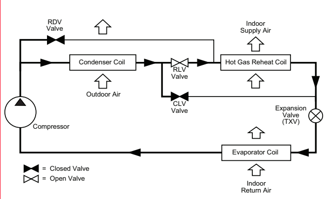
Subcooling Mode (Reheat1) — Perfect Humidity System with 2-Stage Cooling
