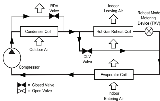
Subcooling Mode (Reheat1) — Perfect Humidity System with Single Stage Cooling
