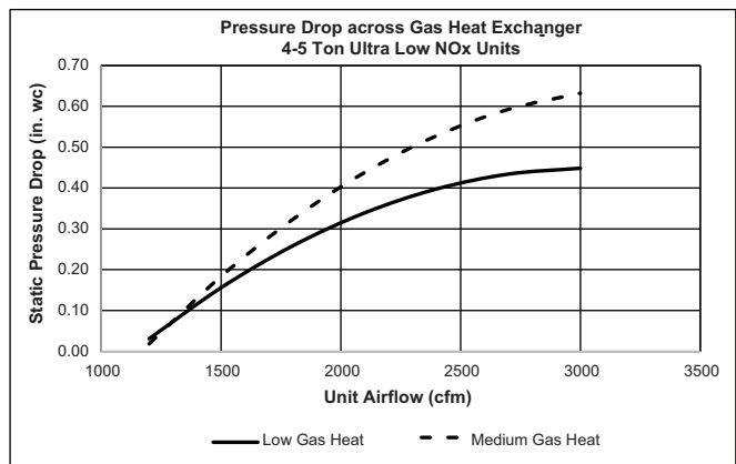
Pressure Drop across Gas Heat Exchanger, 582L Ultra Low NOx — 4 to 5 Ton Units
