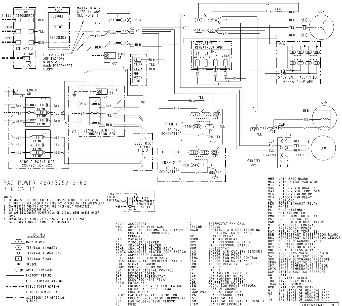
Typical 559L 04-07 Power Wiring Diagram, 460/575-v Unit Shown
