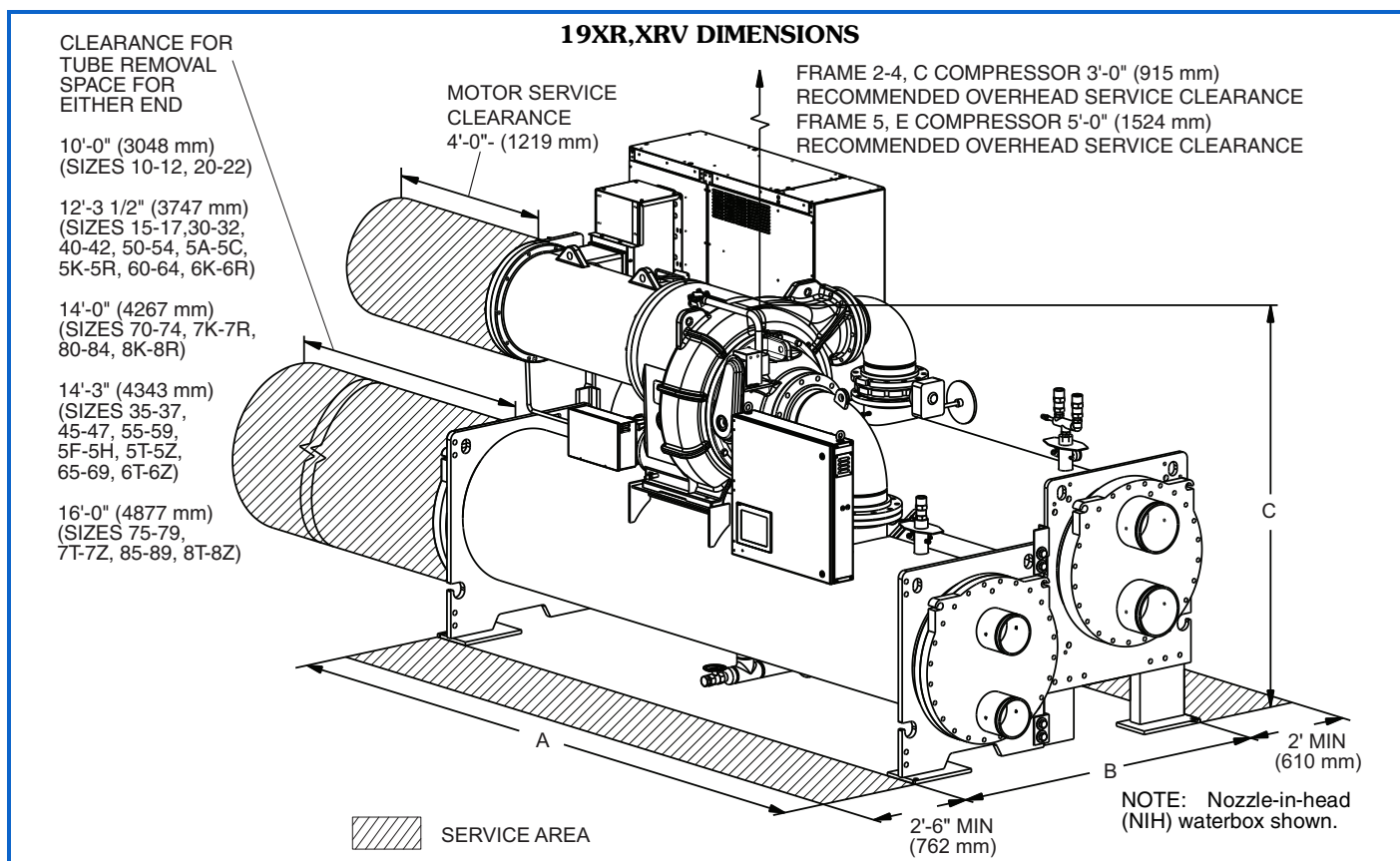
19XR,XRV DIMENSIONS — SINGLE-STAGE COMPRESSOR AND TWO-STAGE COMPRESSOR FRAME SIZE C AND E (MARINE WATERBOX)
