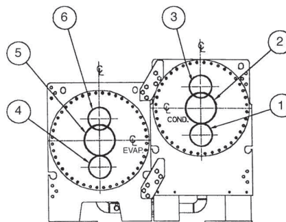
COMPRESSOR END
