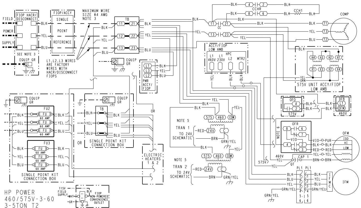
Typical 50GCQ*04-06 Power Wiring Diagram, 460/575-3-60 Unit Shown
