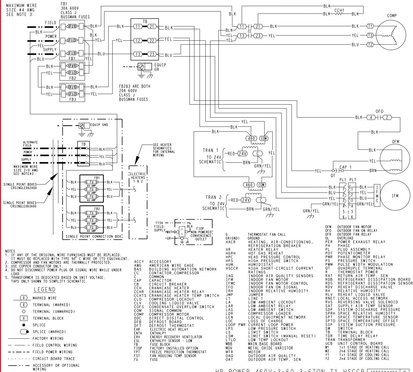
Typical 547L*04-07 Power Wiring Diagram, Electromechanical, 460-3-60 High SCCR Shown
