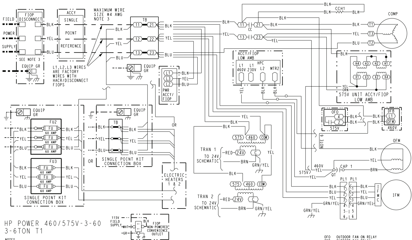
Typical 547L*04-07 Power Wiring Diagram, Electromechanical, 460/575-3-60 Standard SCCR Shown
