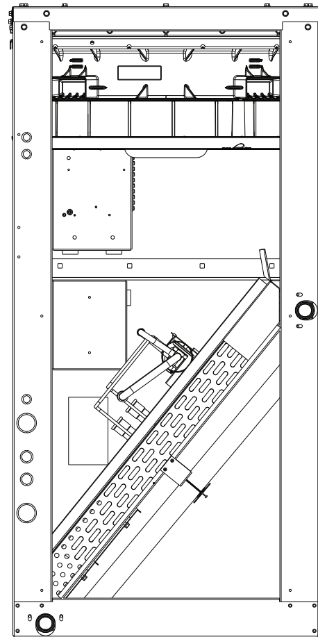
Fig. 33 — Fan Assembly, Side Panel Access (Side Panel Removed)
