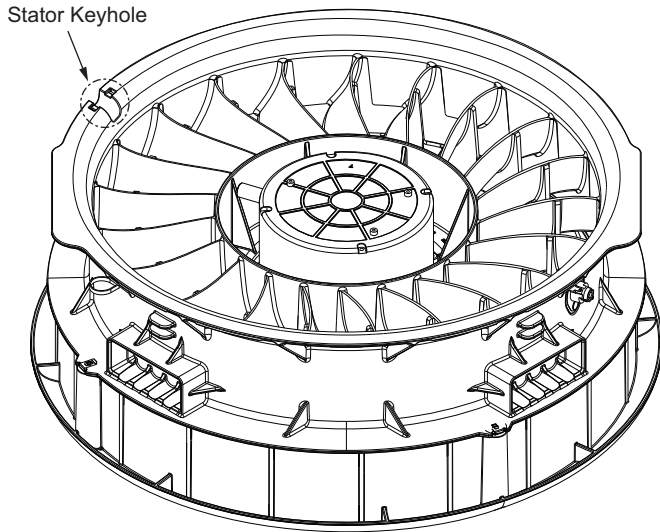
Fig. 36 — Stator Keyhole Location
