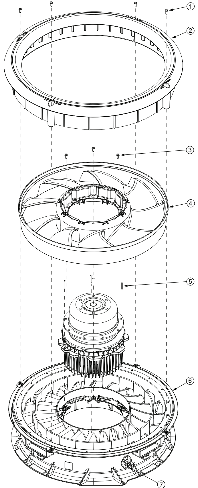
Fig. 35 — Fan Assembly for Units with 3 Hp Motor
