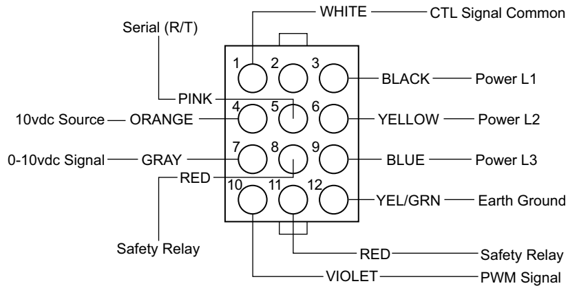
Fig. 27 — ECM Motor Plug Connectors
