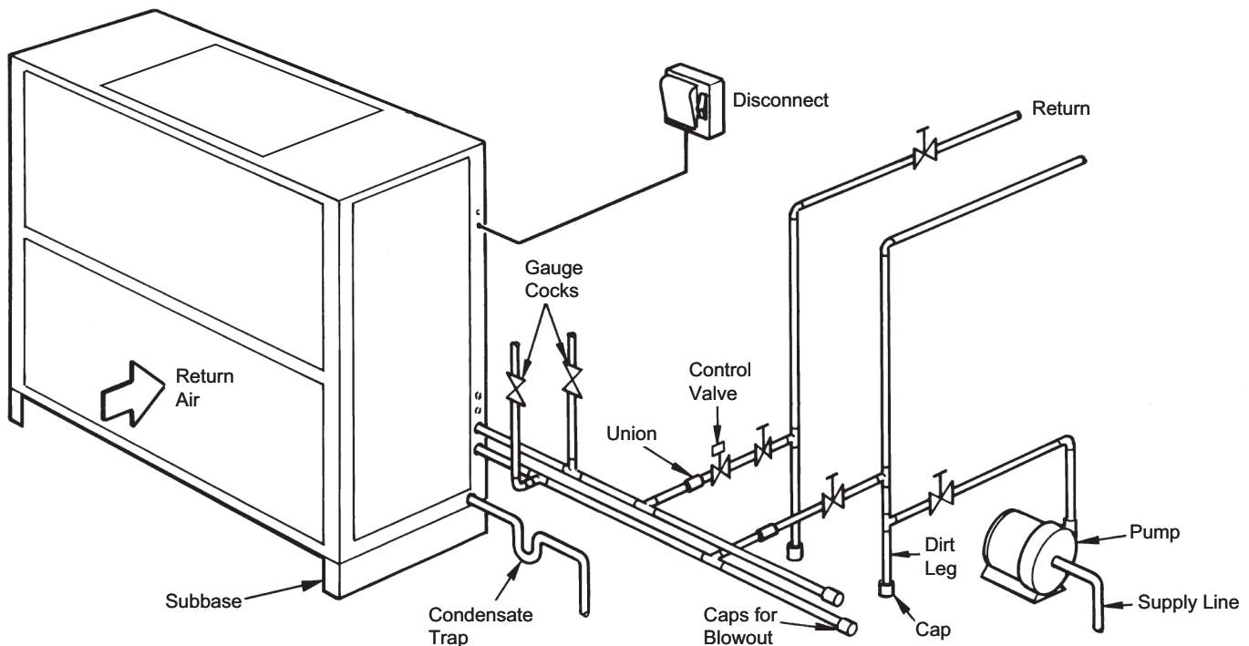
Fig. 10 — Typical 40RLS Chilled Water Piping
