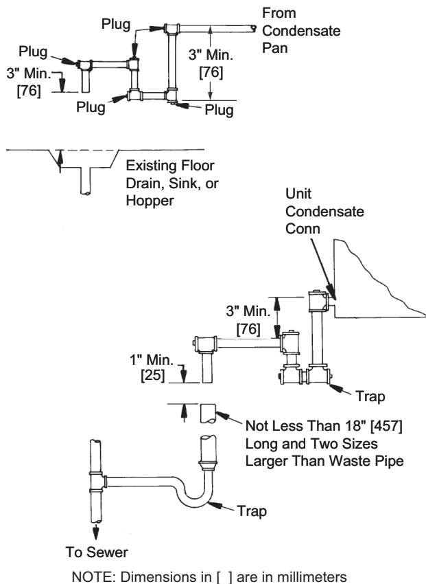
Fig. 11 — Condensate Drain
