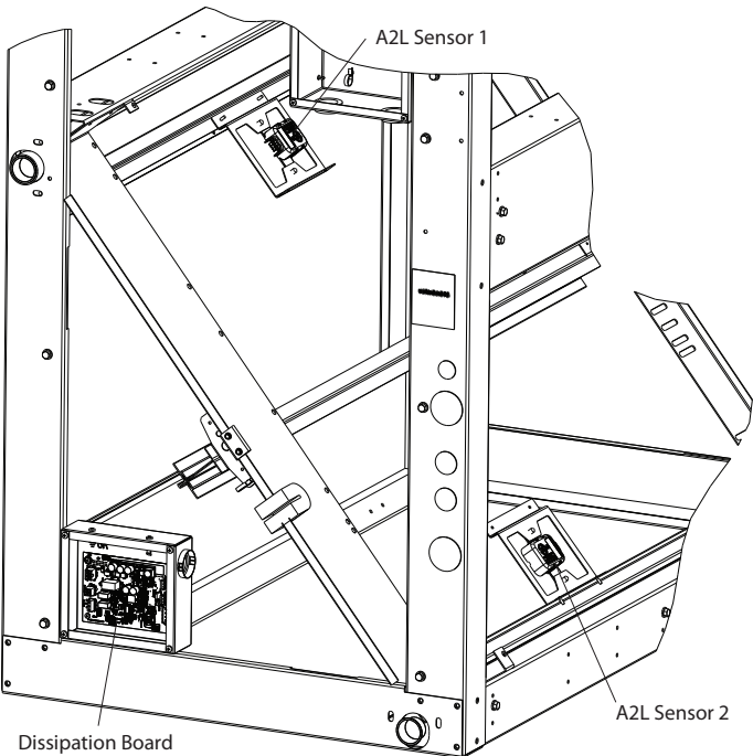
Fig. 18 — Location of A2L Sensors and Dissipation Control Board (Shown with Cover Removed)
