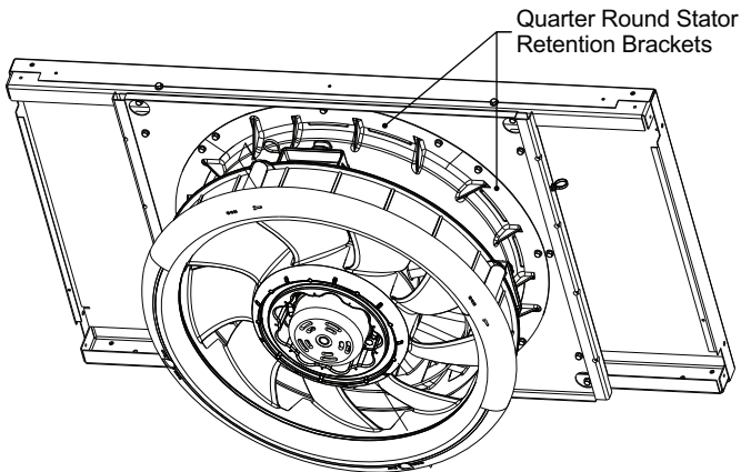
Fig. 32 — Quarter Round Stator Retention Brackets
