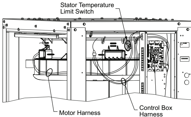
Fig. 31 — Locations of Motor Harness and Stator Temperature Limit Switch
