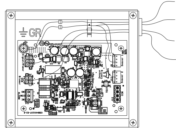
Fig. 20 — Dissipation Control Box
