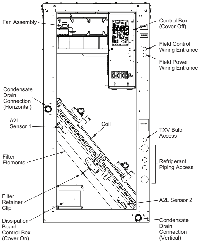
Fig. 14 — Wiring and Service Access (Side Panel Removed)
