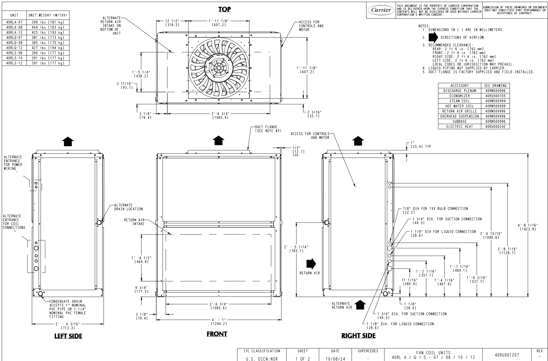
Fig. 2 — 40RL 07-12 Base Unit Dimensions
