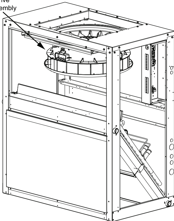
Fig. 26 — Direct-Drive Supply Fan Assembly
