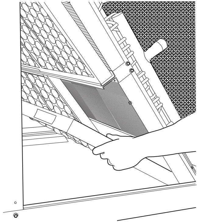
Fig. 41 — Filter Removal/Replacement
