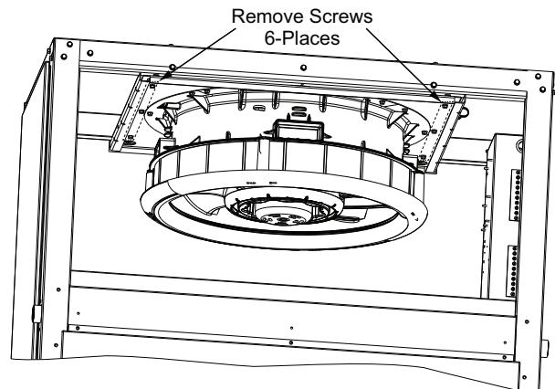
Fig. 37 — Remove Screws from Fan Deck Assembly
