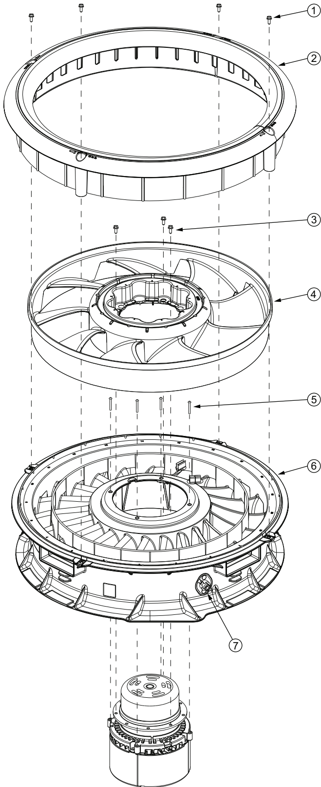
Fig. 34 — Fan Assembly for Units with 2.4 Hp Motor
