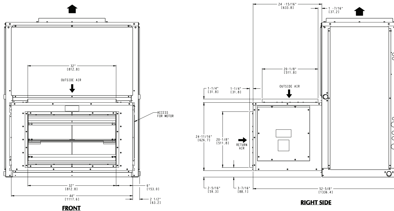
UNIT WITH ECONOMIZER
