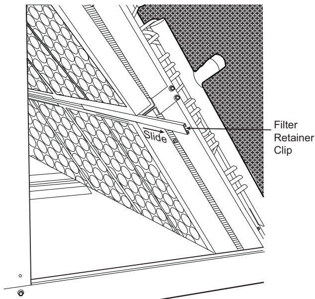
Fig. 40 — Remove Filter Retainer Clip
