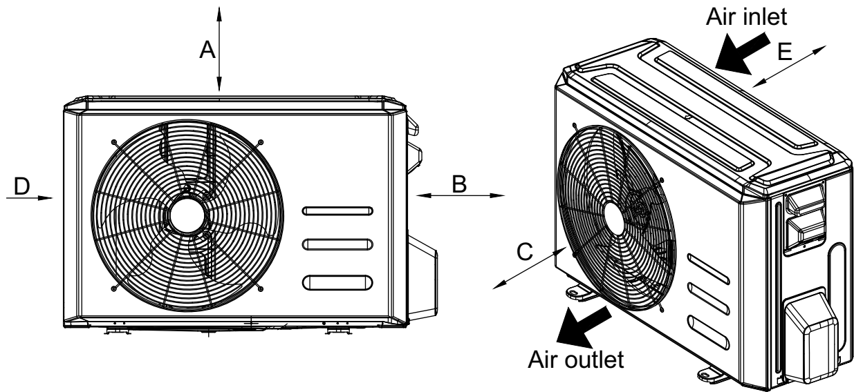
Fig. 5 — Clearances
