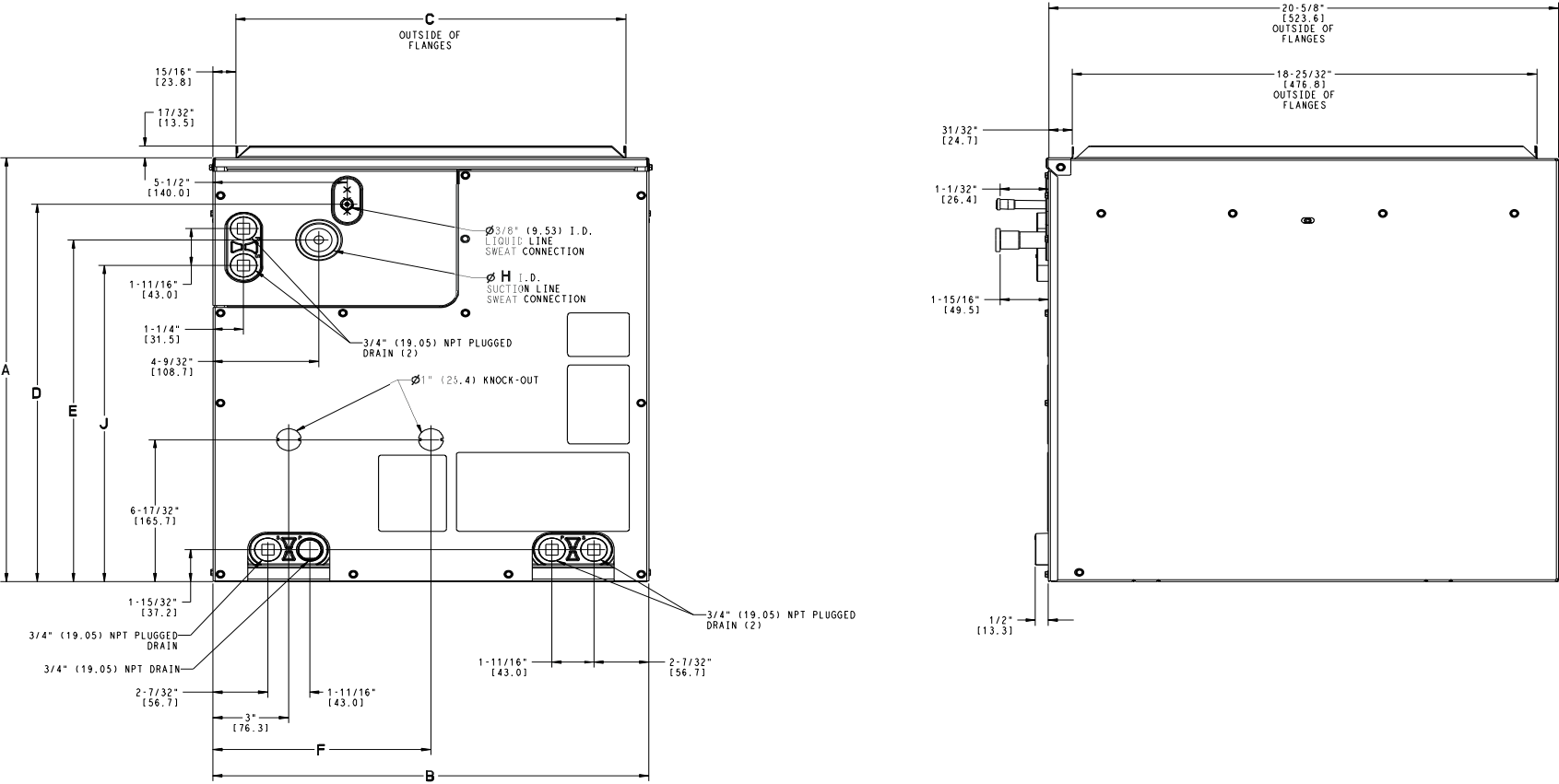
Fig. 9 – CVPMA Dimensions
