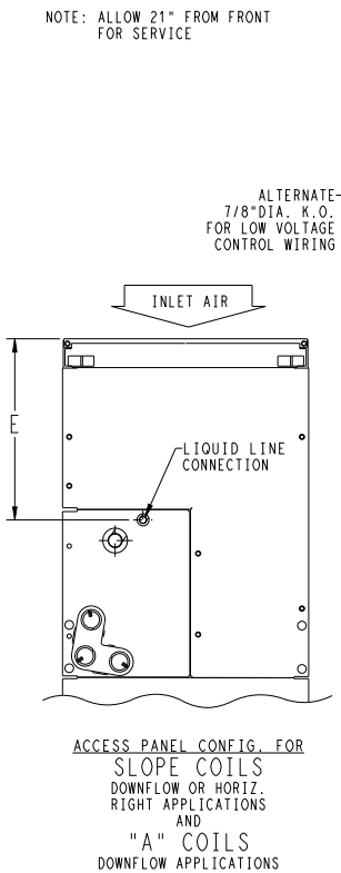
Fig. 1 – Dimensions, sheet 1
