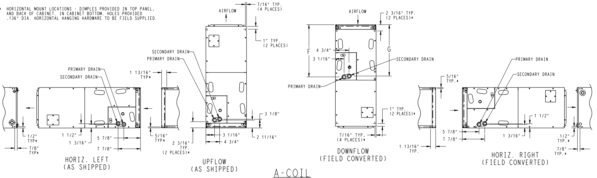
Fig. 2 – Dimensions, sheet 2
