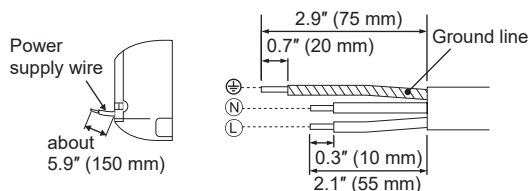
<Stripping length of the power supply wire>
