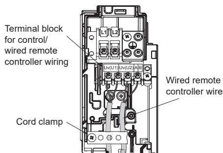
<Connecting wired remote controller wire>
