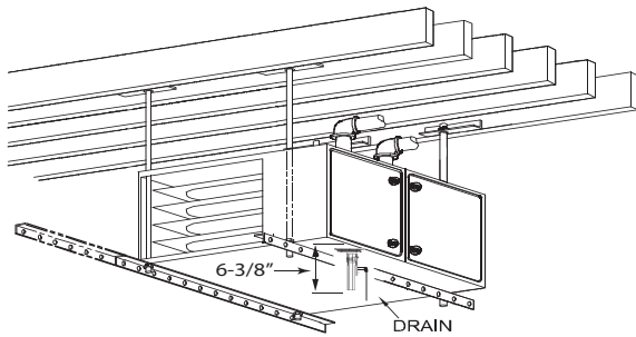
Trap Clearance in Horizontal Application
