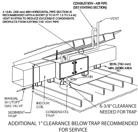
Working Platform for Attic Installation
