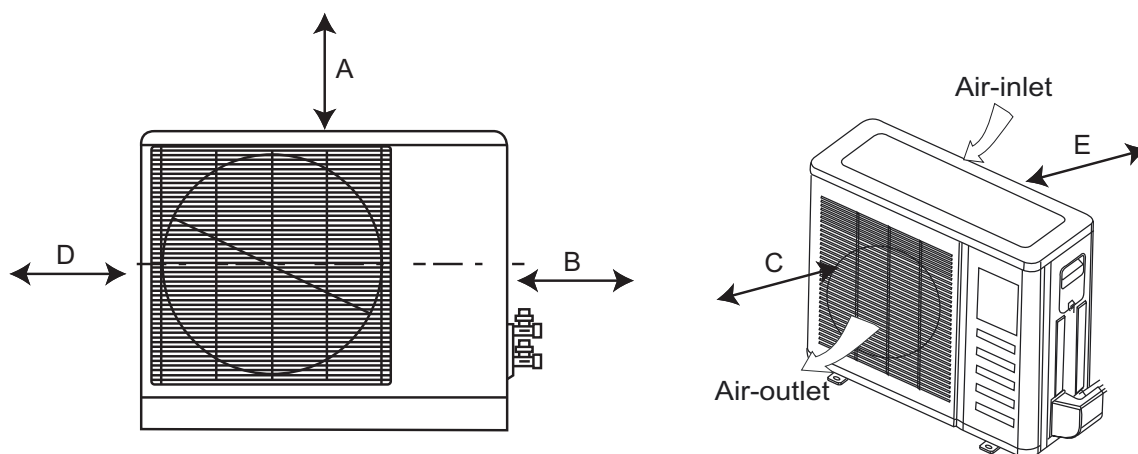
Fig. 9 — Clearances
