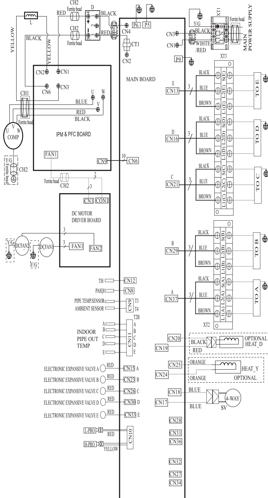
Fig. 16 — Wiring Diagram 48K - 5 Zone Max
