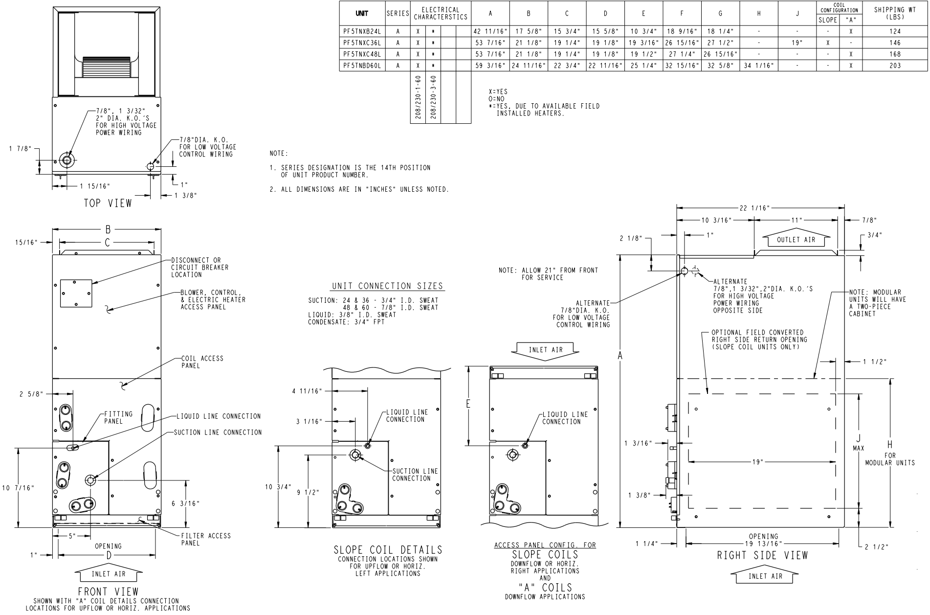
Fig. 1 – Dimensions, sheet 1
