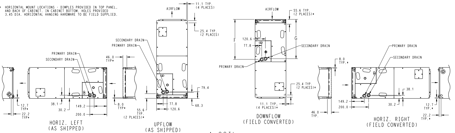
Fig. 4 – Dimensions, sheet 4
