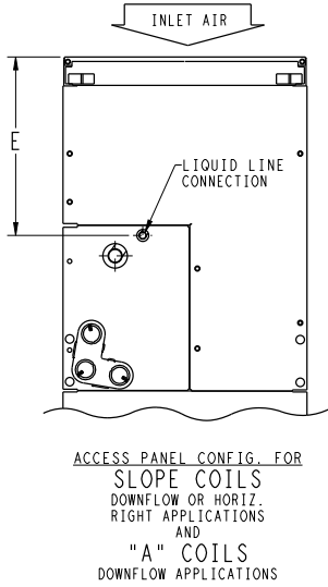
Fig. 3 – Dimensions, sheet 3
