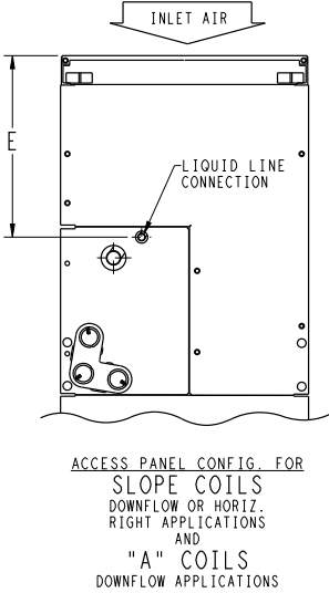
Fig. 3 – Dimensions, sheet 3
