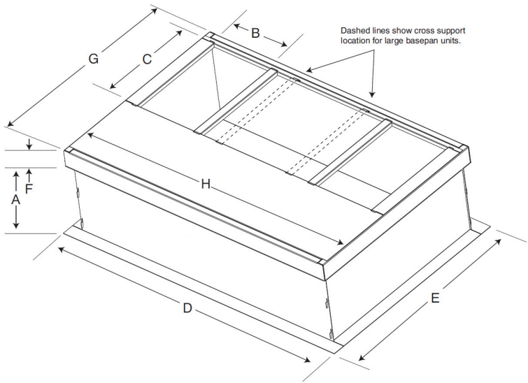
SMALL/COMMON CURB
