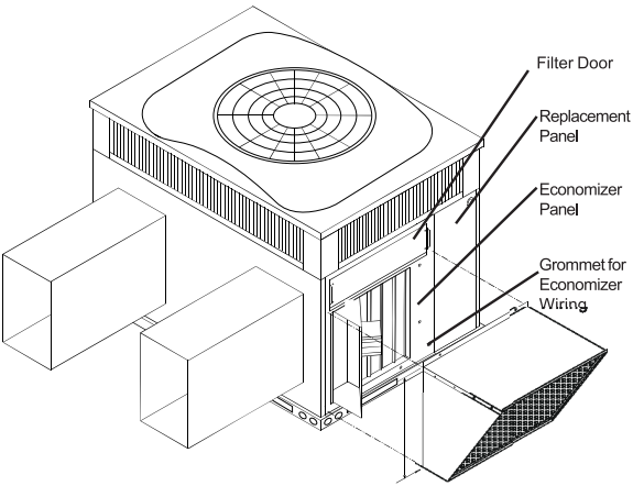
Horizontal Economizer
