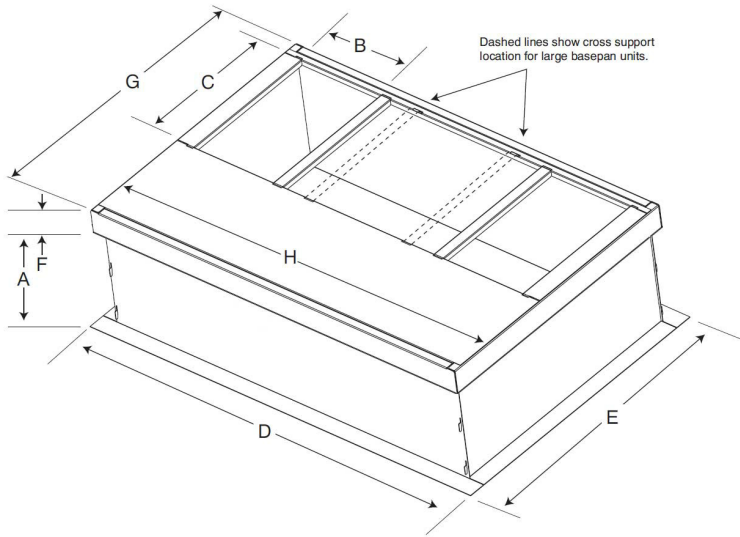
SMALL/COMMON CURB
