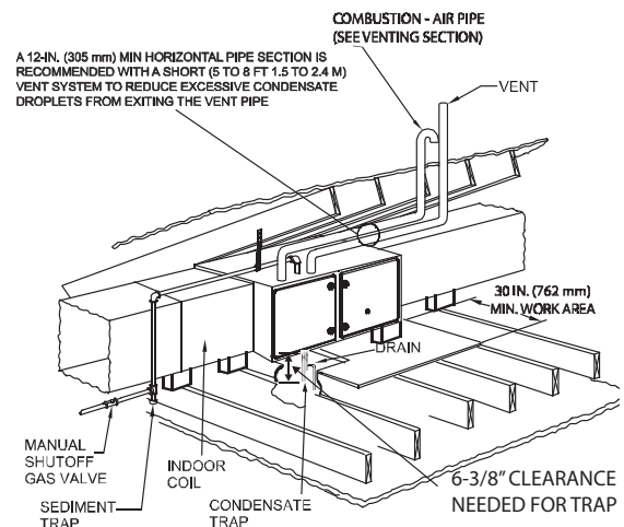
ADDITIONAL 1" CLEARANCE BELOW TRAP RECOMMENDED FOR SERVICE
