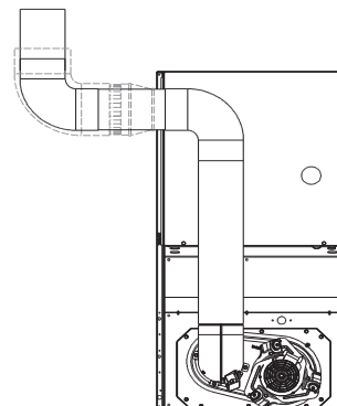
DOWNFLOW
