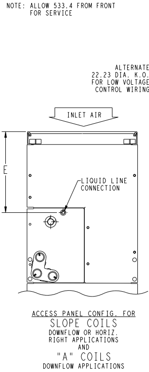
Fig. 3 – Dimensions, sheet 3
