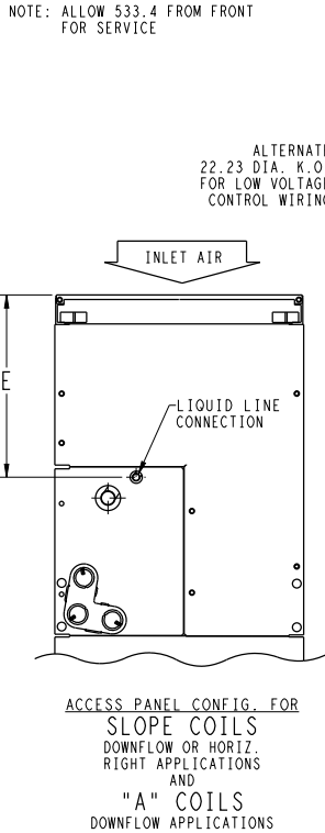
Fig. 3 – Dimensions, sheet 3
