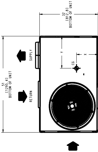
TOP VIEW
