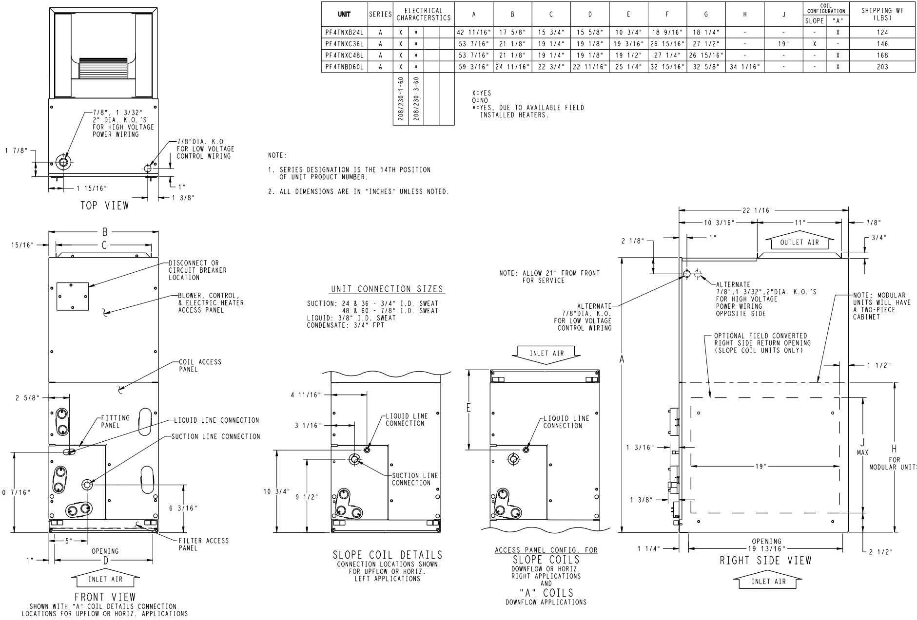
Fig. 1 – Dimensions, sheet 1
