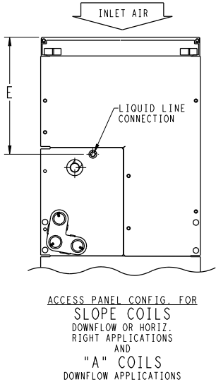
Fig. 3 – Dimensions, sheet 3
