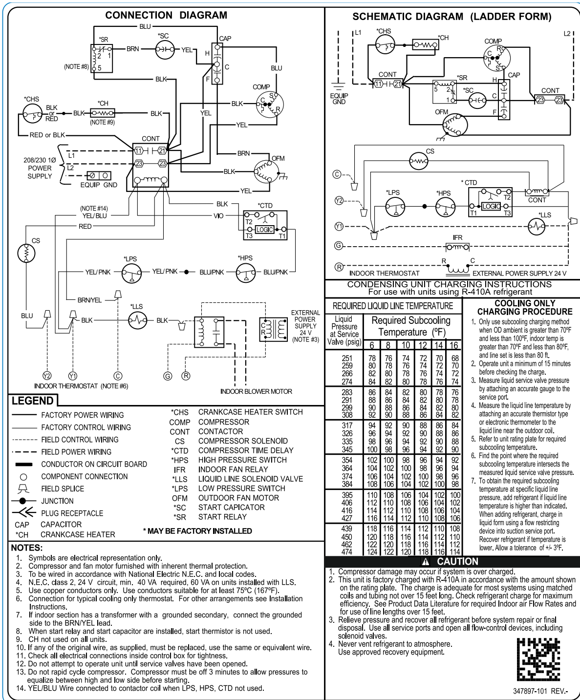
Fig. 1 – 24TPA724-60 Wiring Diagram
