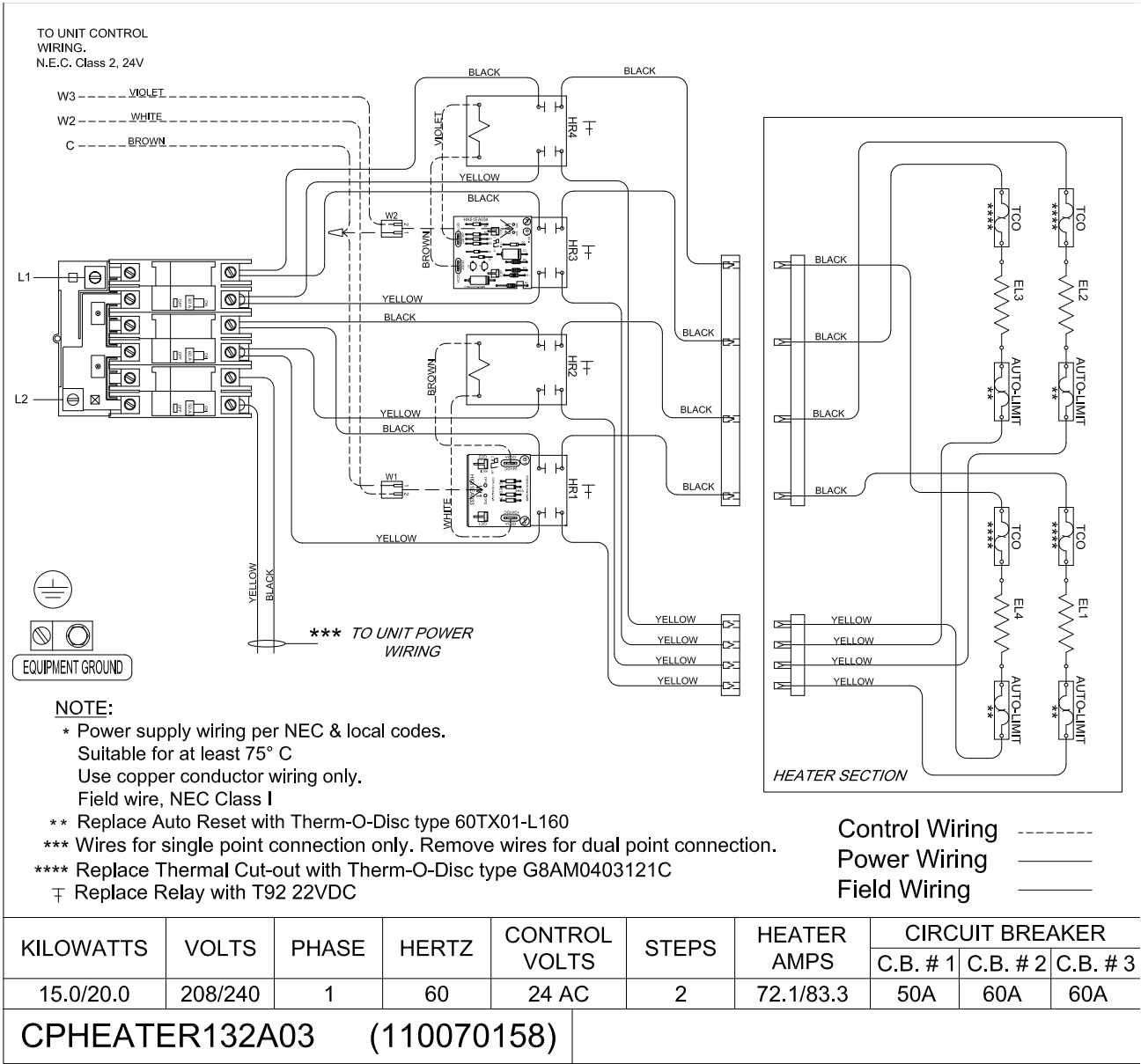
Single-Phase Accessory Electric Heater Wiring
