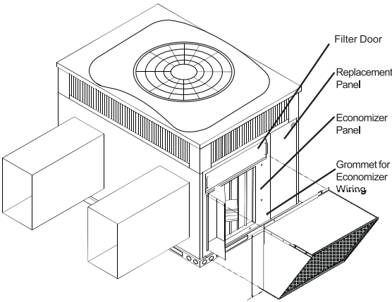
Horizontal Economizer
