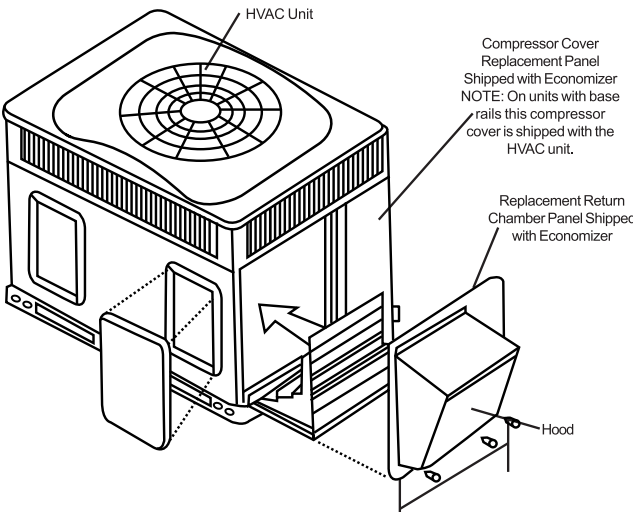
Vertical Economizer
