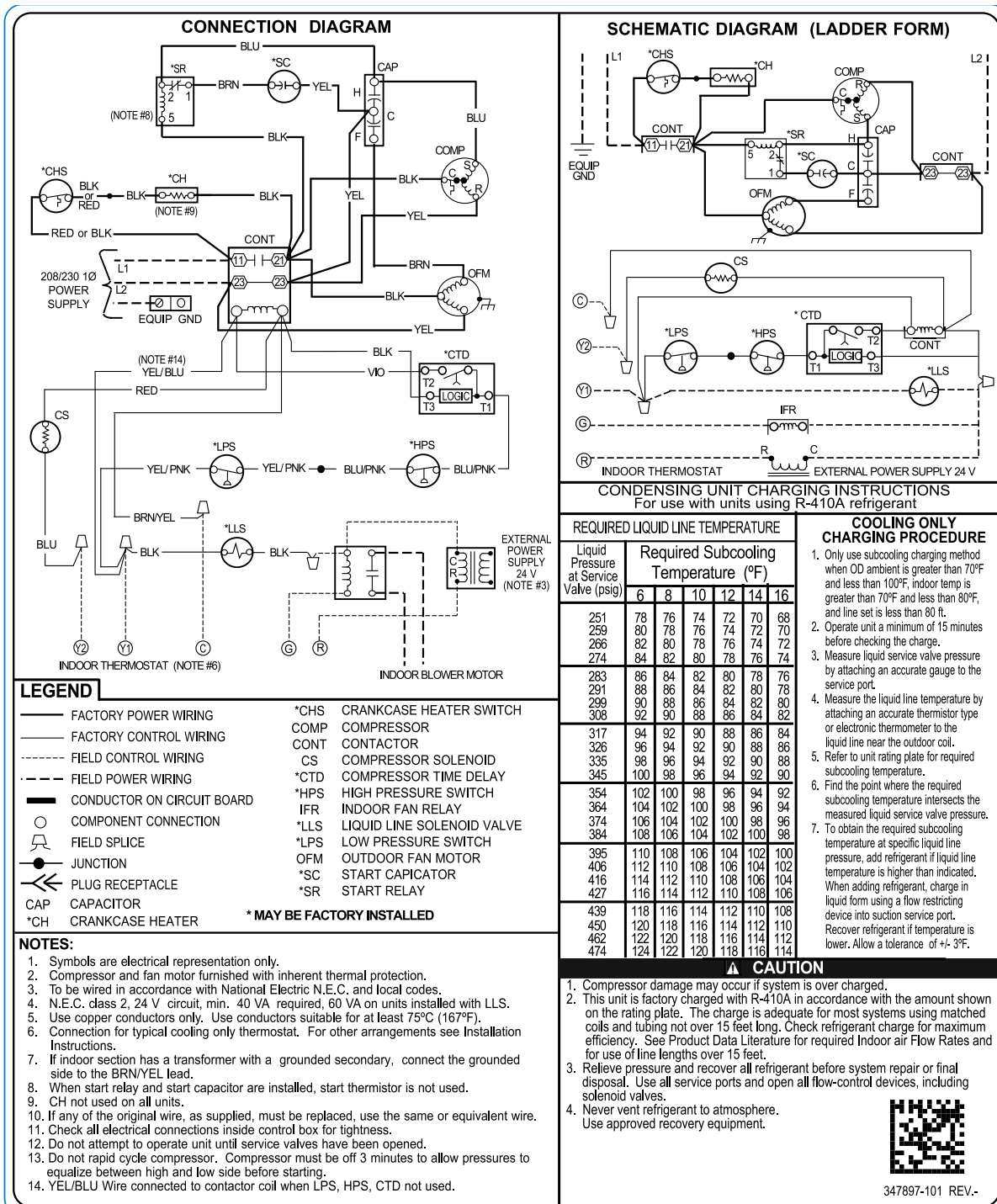
Fig. 1 – 127TAN024-60 Wiring Diagram
