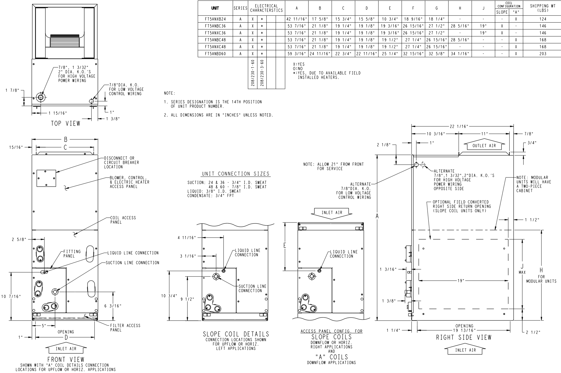
Fig. 1 – Dimensions, sheet 1
