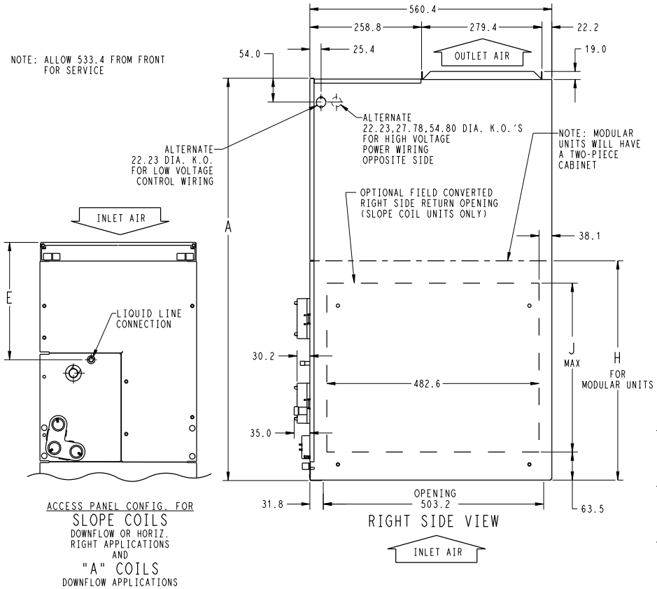
Fig. 3 – Dimensions, sheet 3
