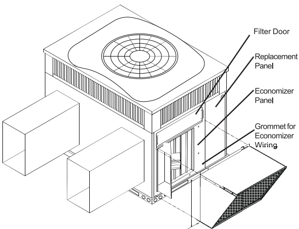
Vertical Economizer
