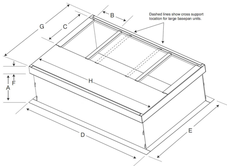
SMALL/COMMON CURB
