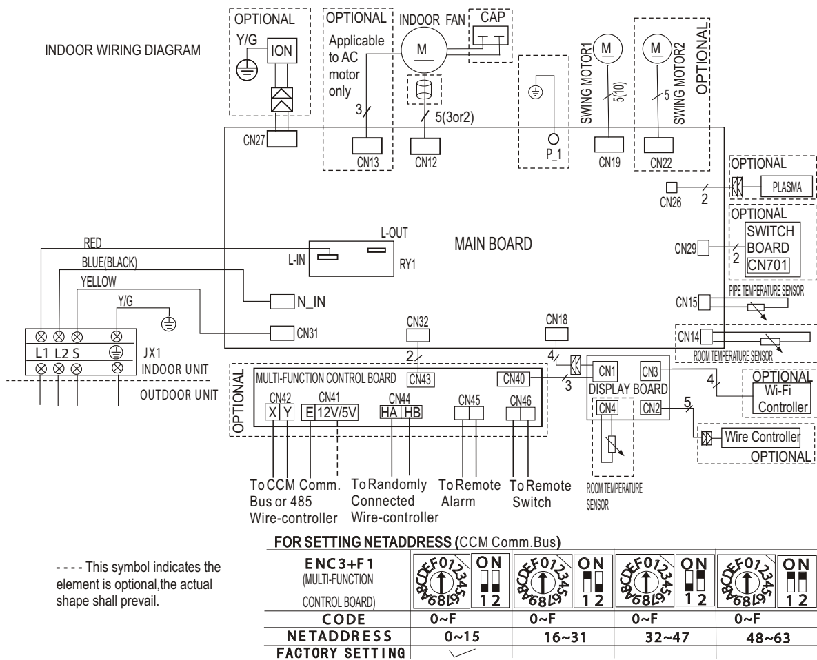
Fig. 12 — Wiring Diagram Sizes 09-24 (208-230V)
